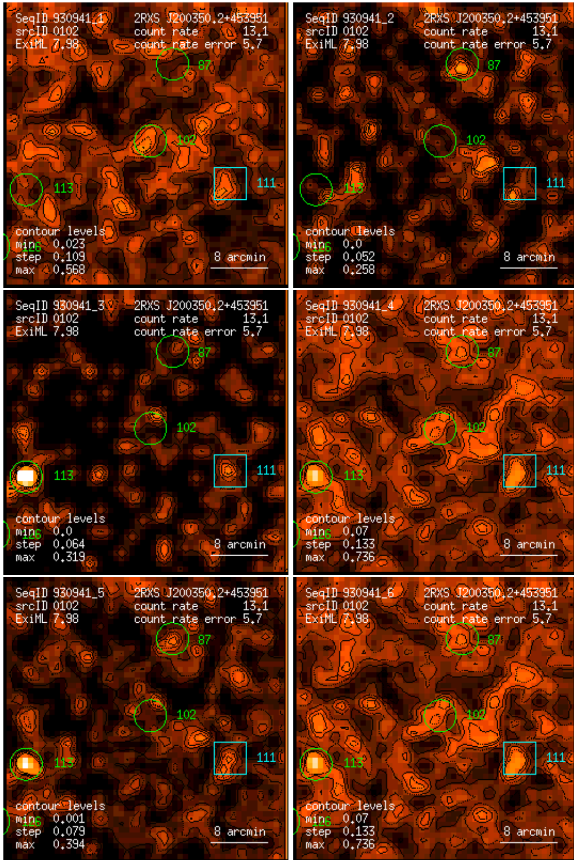
Figure 102: RASS 930941: detection 0102: band rate images, Gaussian filter: (1) PSPC channels 11 – 41, (2) 52 – 90, (3) 91 – 201, (4) 11 – 235, (5) 52 – 201, (6) 11 – 201. Broad band rates in counts/ks. Band rate contour levels in counts/ks/arcmin 2 .
