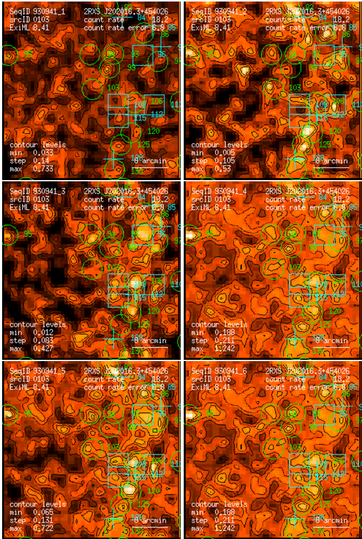
Figure 103: RASS 930941: detection 0103: band rate images, Gaussian filter: (1) PSPC channels 11 – 41, (2) 52 – 90, (3) 91 – 201, (4) 11 – 235, (5) 52 – 201, (6) 11 – 201. Broad band rates in counts/ks. Band rate contour levels in counts/ks/arcmin 2 .
