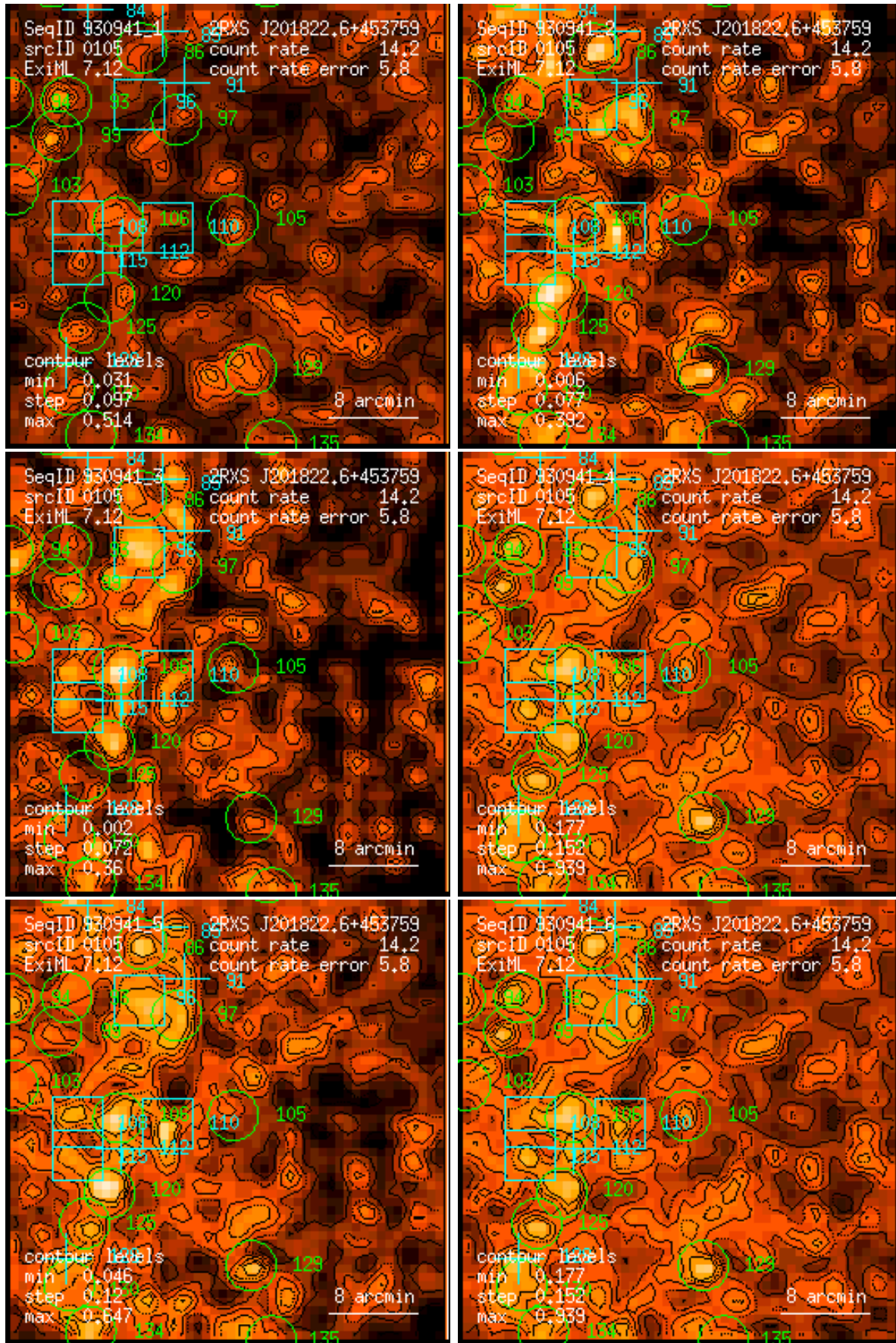
Figure 105: RASS 930941: detection 0105: band rate images, Gaussian filter: (1) PSPC channels 11 – 41, (2) 52 – 90, (3) 91 – 201, (4) 11 – 235, (5) 52 – 201, (6) 11 – 201. Broad band rates in counts/ks. Band rate contour levels in counts/ks/arcmin 2 .
