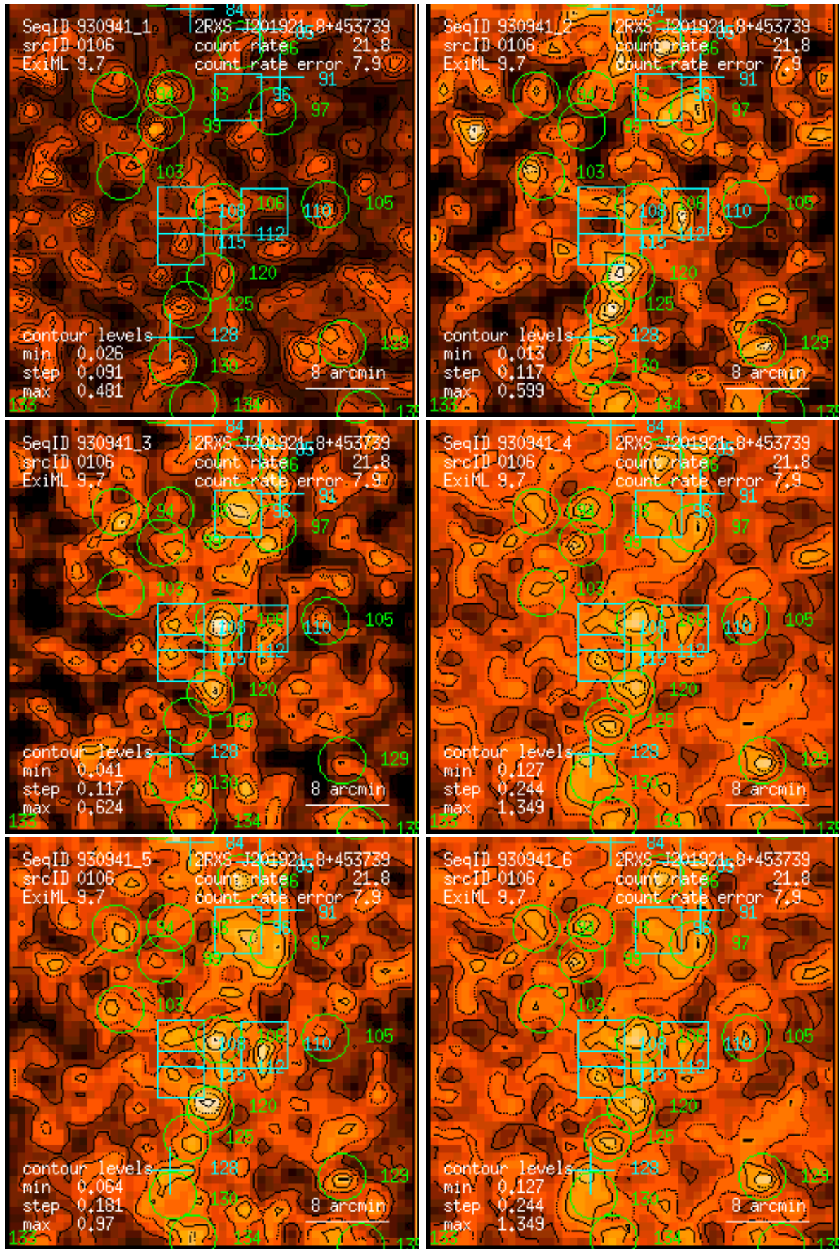
Figure 106: RASS 930941: detection 0106: band rate images, Gaussian filter: (1) PSPC channels 11 – 41, (2) 52 – 90, (3) 91 – 201, (4) 11 – 235, (5) 52 – 201, (6) 11 – 201. Broad band rates in counts/ks. Band rate contour levels in counts/ks/arcmin 2 .
