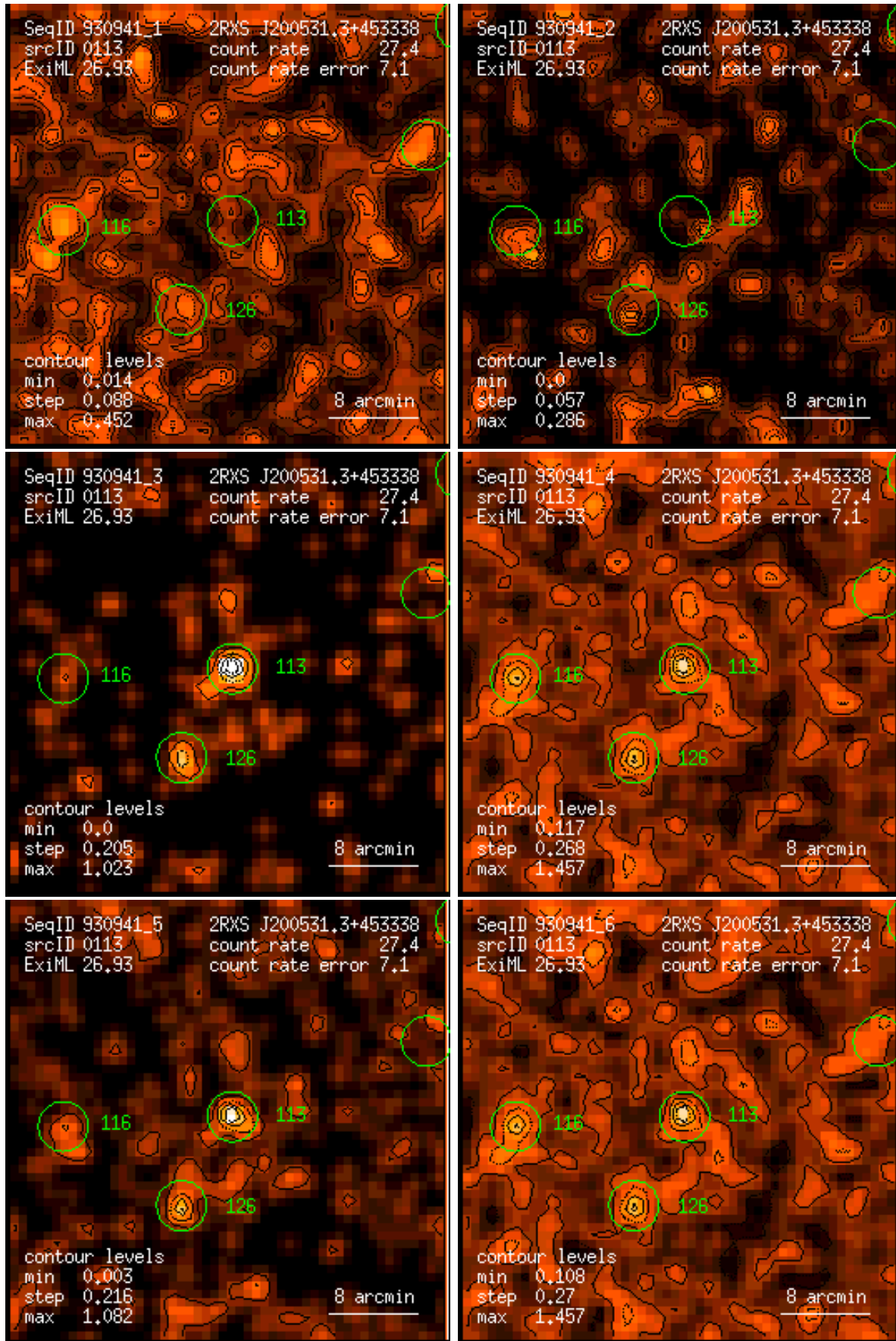
Figure 113: RASS 930941: detection 0113: band rate images, Gaussian filter: (1) PSPC channels 11 – 41, (2) 52 – 90, (3) 91 – 201, (4) 11 – 235, (5) 52 – 201, (6) 11 – 201. Broad band rates in counts/ks. Band rate contour levels in counts/ks/arcmin 2 .
