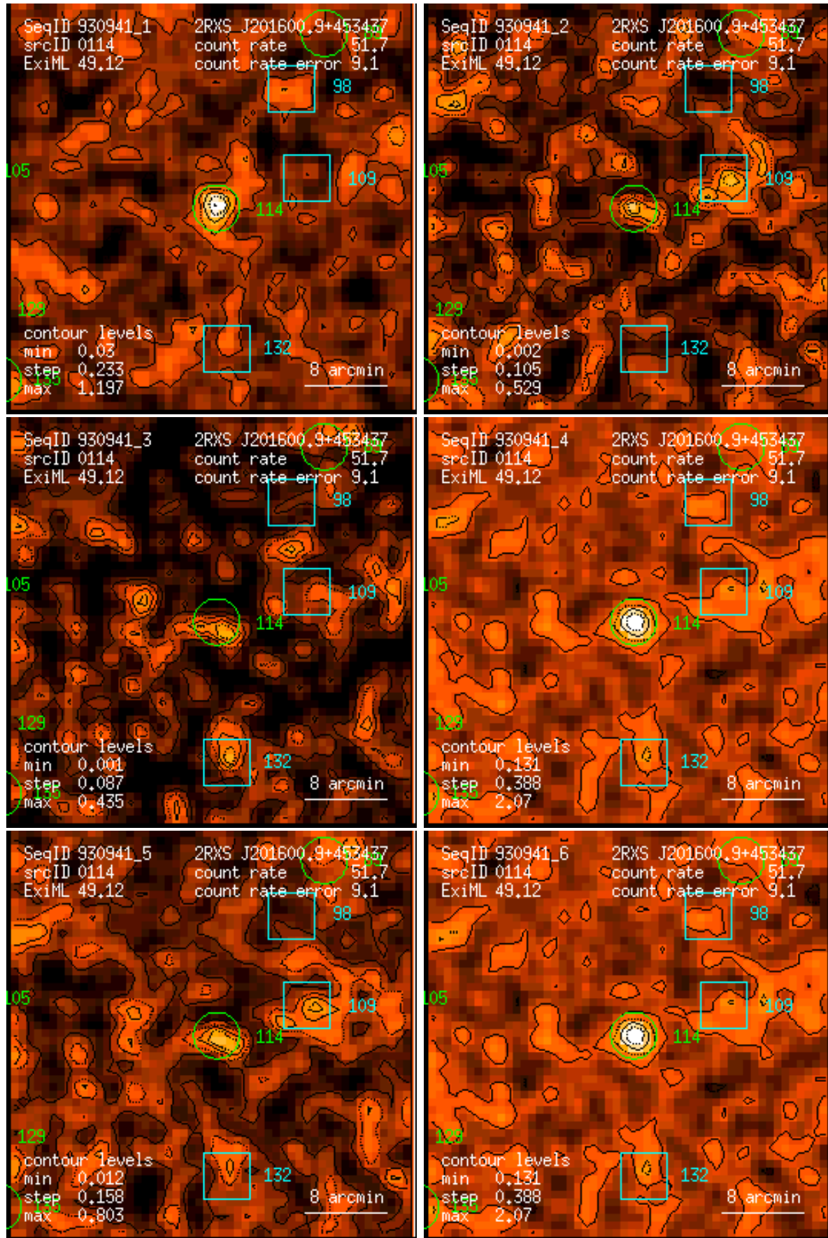
Figure 114: RASS 930941: detection 0114: band rate images, Gaussian filter: (1) PSPC channels 11 – 41, (2) 52 – 90, (3) 91 – 201, (4) 11 – 235, (5) 52 – 201, (6) 11 – 201. Broad band rates in counts/ks. Band rate contour levels in counts/ks/arcmin 2 .
