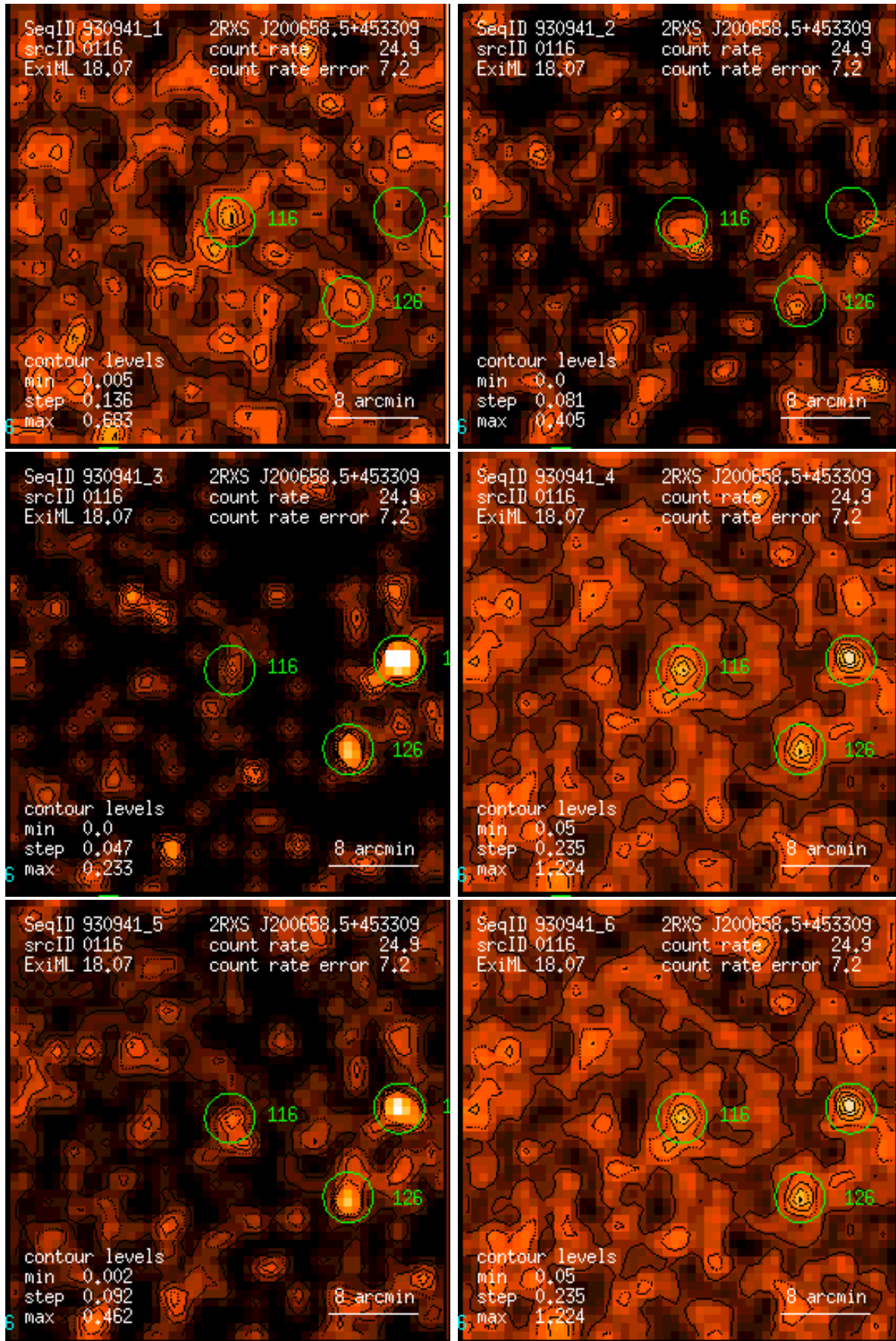
Figure 116: RASS 930941: detection 0116: band rate images, Gaussian filter: (1) PSPC channels 11 – 41, (2) 52 – 90, (3) 91 – 201, (4) 11 – 235, (5) 52 – 201, (6) 11 – 201. Broad band rates in counts/ks. Band rate contour levels in counts/ks/arcmin 2 .
