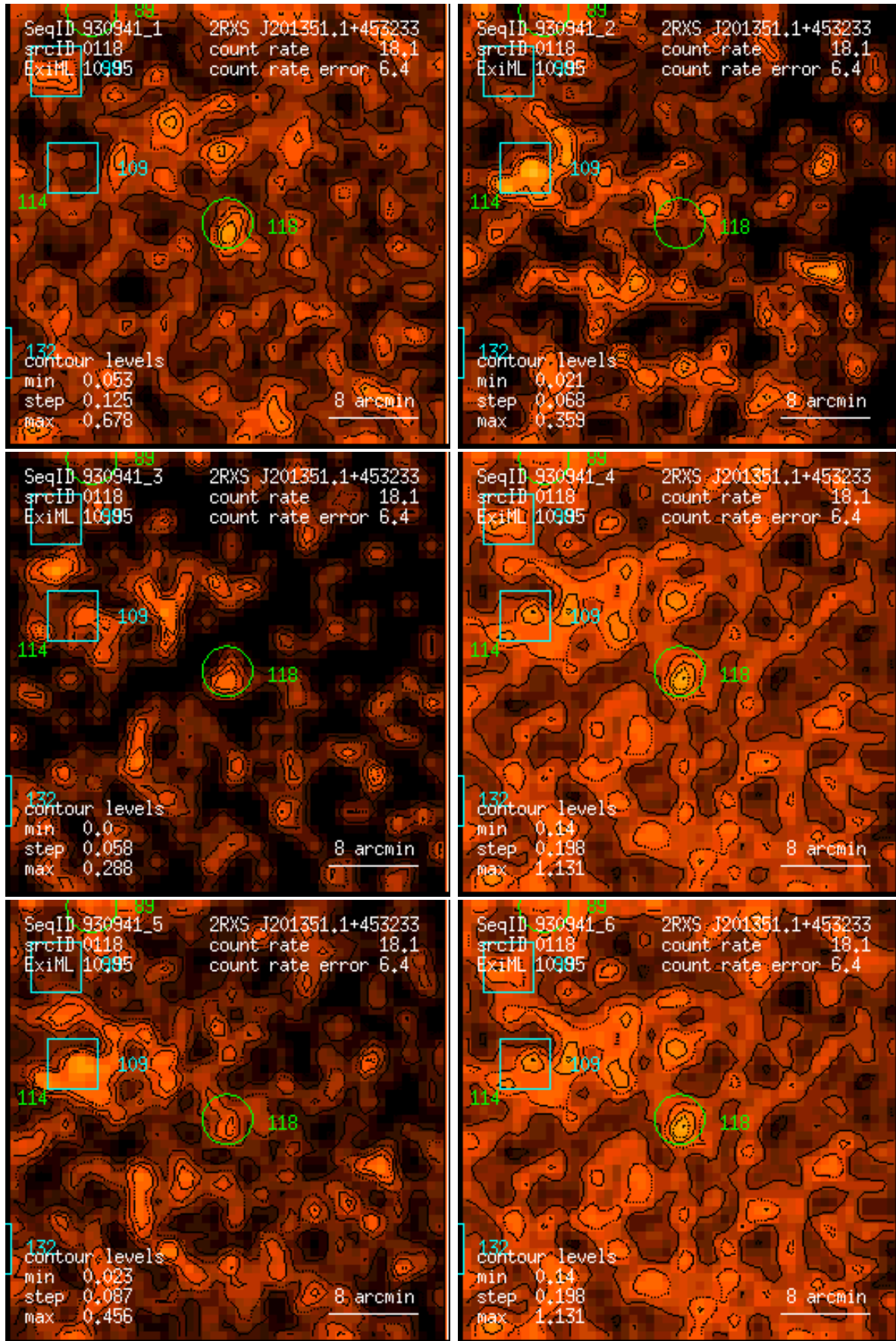
Figure 118: RASS 930941: detection 0118: band rate images, Gaussian filter: (1) PSPC channels 11 – 41, (2) 52 – 90, (3) 91 – 201, (4) 11 – 235, (5) 52 – 201, (6) 11 – 201. Broad band rates in counts/ks. Band rate contour levels in counts/ks/arcmin 2 .
