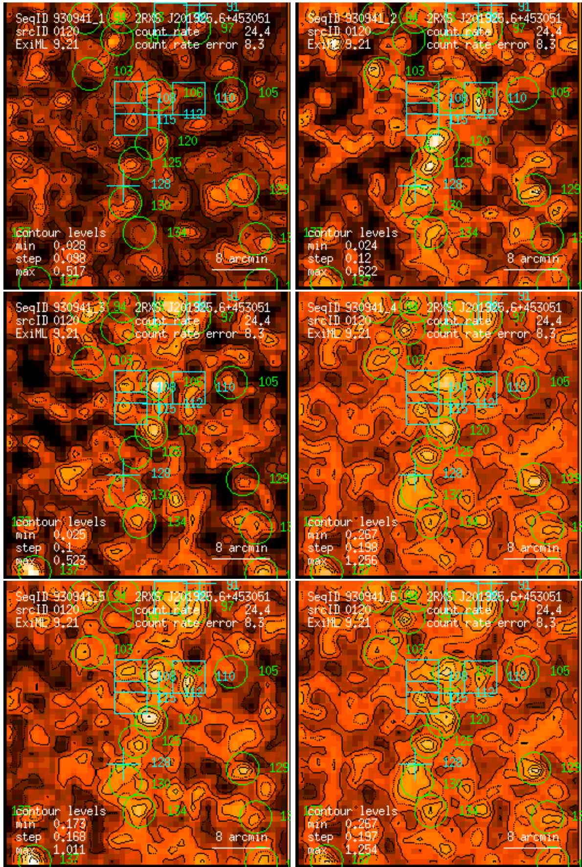
Figure 120: RASS 930941: detection 0120: band rate images, Gaussian filter: (1) PSPC channels 11 – 41, (2) 52 – 90, (3) 91 – 201, (4) 11 – 235, (5) 52 – 201, (6) 11 – 201. Broad band rates in counts/ks. Band rate contour levels in counts/ks/arcmin 2 .
