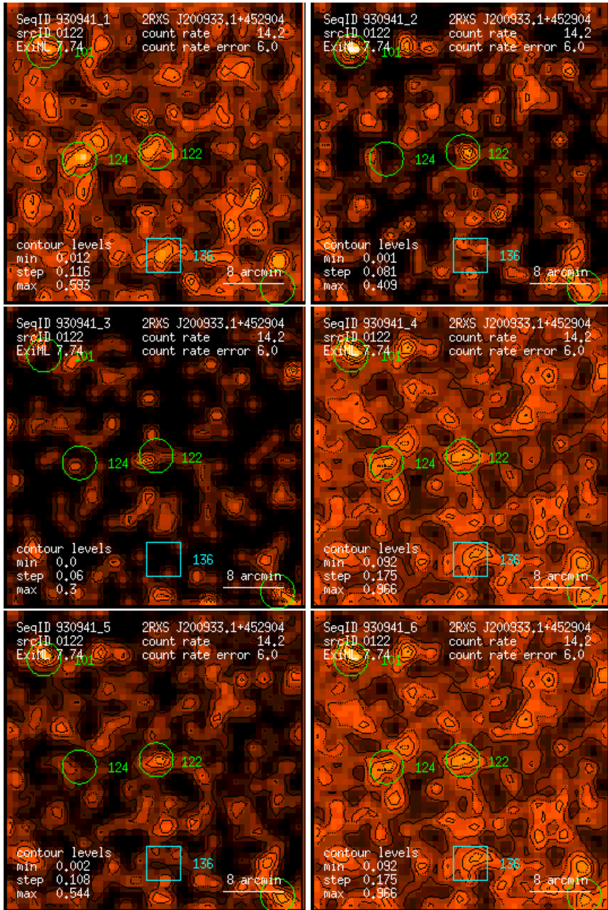
Figure 122: RASS 930941: detection 0122: band rate images, Gaussian filter: (1) PSPC channels 11 – 41, (2) 52 – 90, (3) 91 – 201, (4) 11 – 235, (5) 52 – 201, (6) 11 – 201. Broad band rates in counts/ks. Band rate contour levels in counts/ks/arcmin 2 .
