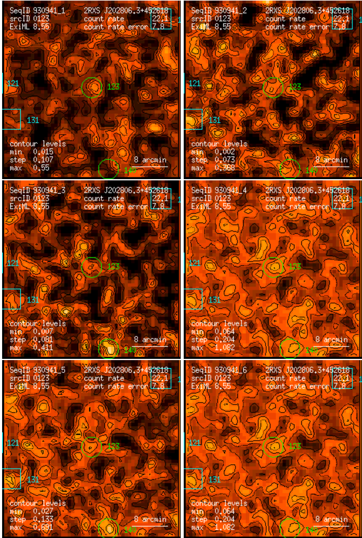
Figure 123: RASS 930941: detection 0123: band rate images, Gaussian filter: (1) PSPC channels 11 – 41, (2) 52 – 90, (3) 91 – 201, (4) 11 – 235, (5) 52 – 201, (6) 11 – 201. Broad band rates in counts/ks. Band rate contour levels in counts/ks/arcmin 2 .
