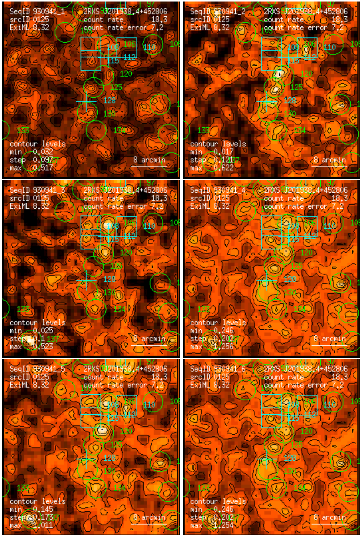
Figure 125: RASS 930941: detection 0125: band rate images, Gaussian filter: (1) PSPC channels 11 – 41, (2) 52 – 90, (3) 91 – 201, (4) 11 – 235, (5) 52 – 201, (6) 11 – 201. Broad band rates in counts/ks. Band rate contour levels in counts/ks/arcmin 2 .
