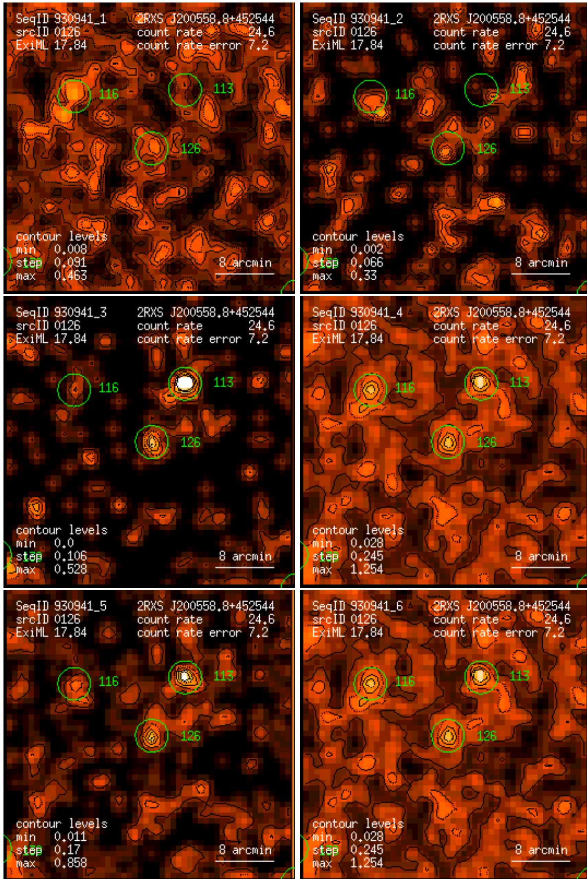
Figure 126: RASS 930941: detection 0126: band rate images, Gaussian filter: (1) PSPC channels 11 – 41, (2) 52 – 90, (3) 91 – 201, (4) 11 – 235, (5) 52 – 201, (6) 11 – 201. Broad band rates in counts/ks. Band rate contour levels in counts/ks/arcmin 2 .
