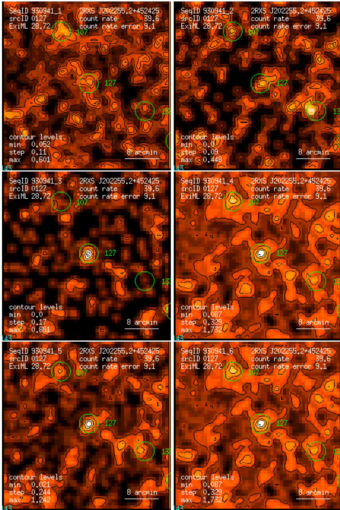
Figure 127: RASS 930941: detection 0127: band rate images, Gaussian filter: (1) PSPC channels 11 – 41, (2) 52 – 90, (3) 91 – 201, (4) 11 – 235, (5) 52 – 201, (6) 11 – 201. Broad band rates in counts/ks. Band rate contour levels in counts/ks/arcmin 2 .
