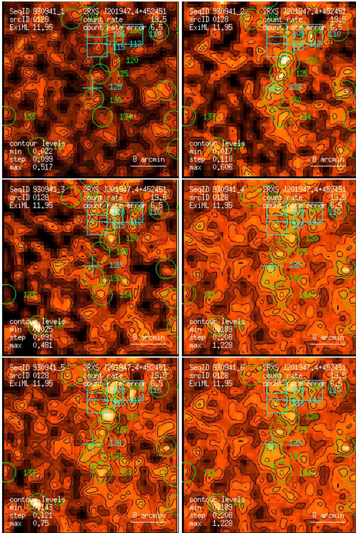
Figure 128: RASS 930941: detection 0128: band rate images, Gaussian filter: (1) PSPC channels 11 – 41, (2) 52 – 90, (3) 91 – 201, (4) 11 – 235, (5) 52 – 201, (6) 11 – 201. Broad band rates in counts/ks. Band rate contour levels in counts/ks/arcmin 2 .
