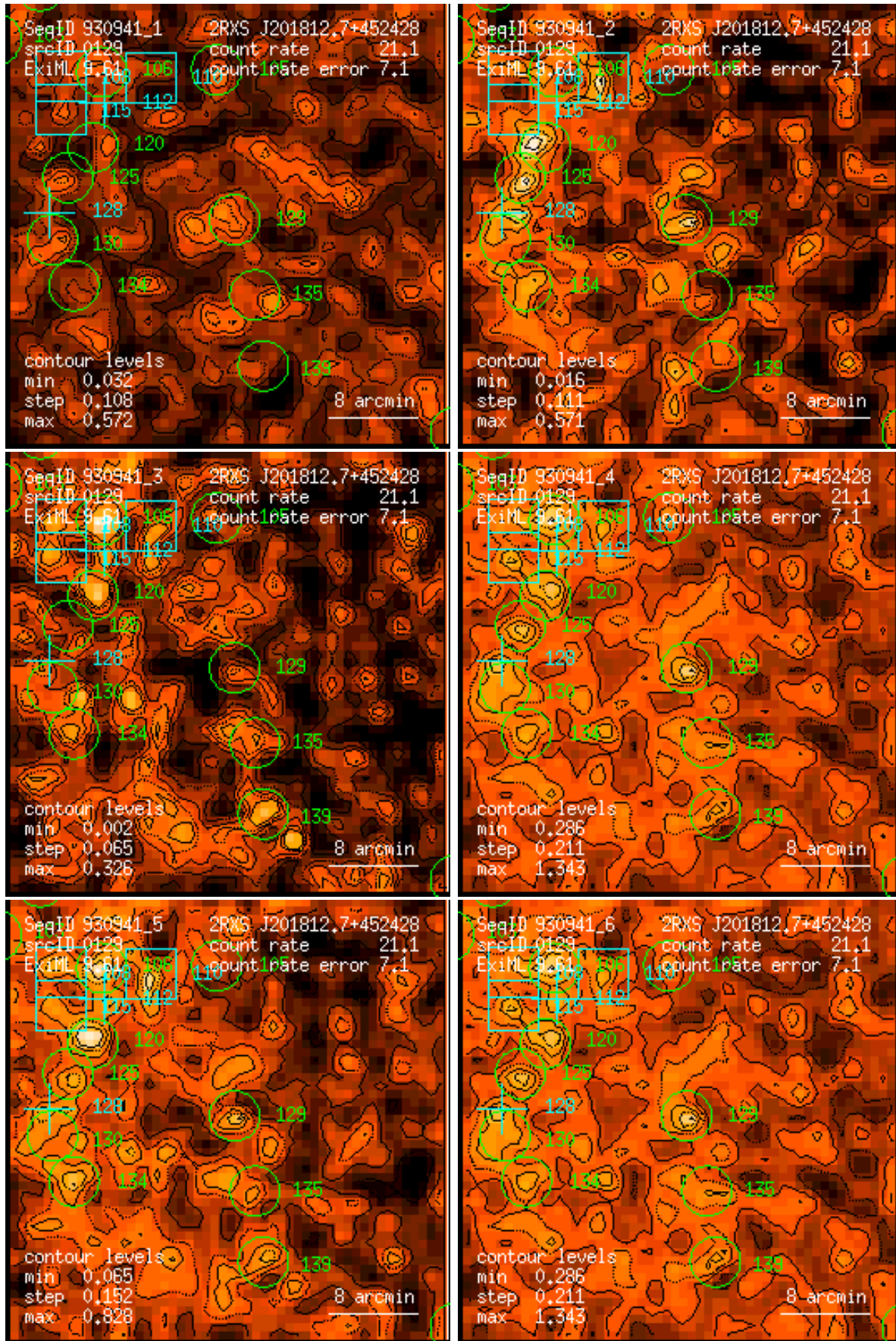
Figure 129: RASS 930941: detection 0129: band rate images, Gaussian filter: (1) PSPC channels 11 – 41, (2) 52 – 90, (3) 91 – 201, (4) 11 – 235, (5) 52 – 201, (6) 11 – 201. Broad band rates in counts/ks. Band rate contour levels in counts/ks/arcmin 2 .
