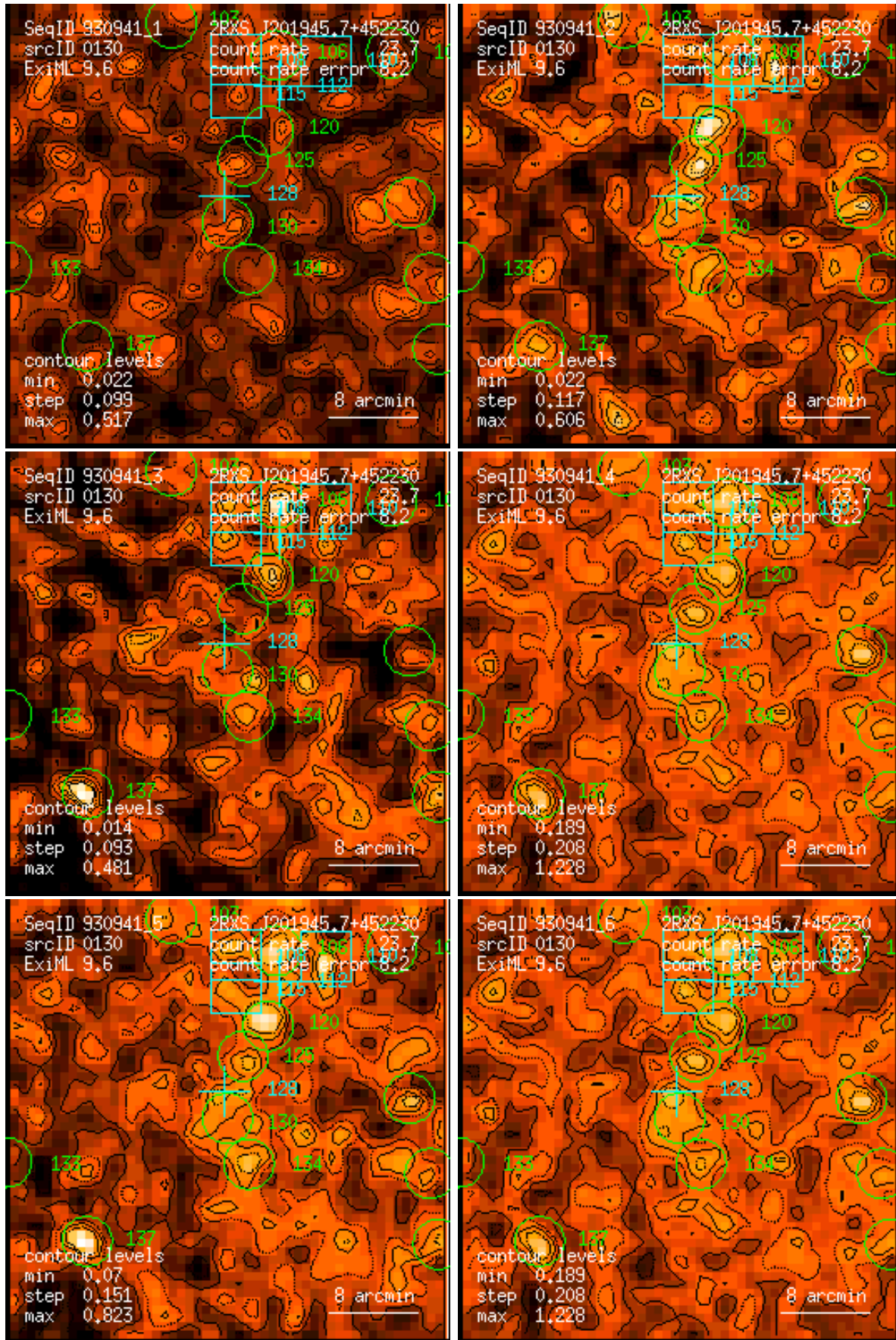
Figure 130: RASS 930941: detection 0130: band rate images, Gaussian filter: (1) PSPC channels 11 – 41, (2) 52 – 90, (3) 91 – 201, (4) 11 – 235, (5) 52 – 201, (6) 11 – 201. Broad band rates in counts/ks. Band rate contour levels in counts/ks/arcmin 2 .
