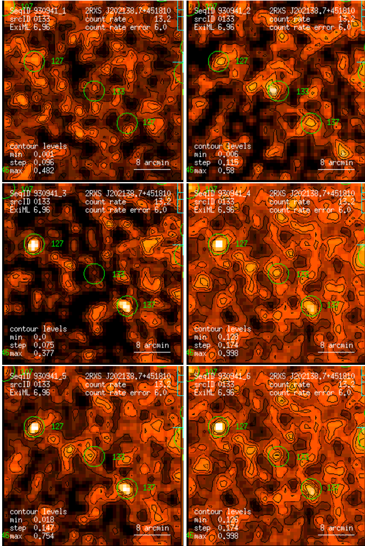
Figure 133: RASS 930941: detection 0133: band rate images, Gaussian filter: (1) PSPC channels 11 – 41, (2) 52 – 90, (3) 91 – 201, (4) 11 – 235, (5) 52 – 201, (6) 11 – 201. Broad band rates in counts/ks. Band rate contour levels in counts/ks/arcmin 2 .
