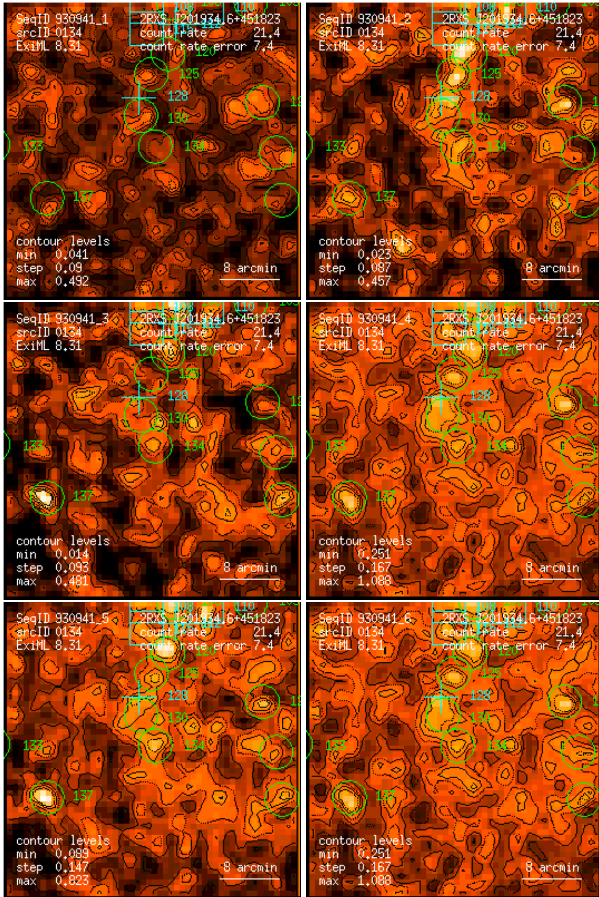
Figure 134: RASS 930941: detection 0134: band rate images, Gaussian filter: (1) PSPC channels 11 – 41, (2) 52 – 90, (3) 91 – 201, (4) 11 – 235, (5) 52 – 201, (6) 11 – 201. Broad band rates in counts/ks. Band rate contour levels in counts/ks/arcmin 2 .
