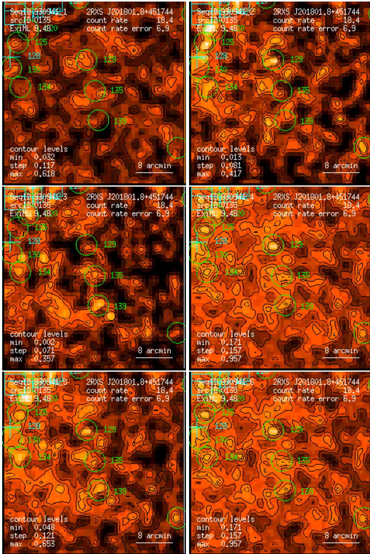
Figure 135: RASS 930941: detection 0135: band rate images, Gaussian filter: (1) PSPC channels 11 – 41, (2) 52 – 90, (3) 91 – 201, (4) 11 – 235, (5) 52 – 201, (6) 11 – 201. Broad band rates in counts/ks. Band rate contour levels in counts/ks/arcmin 2 .
