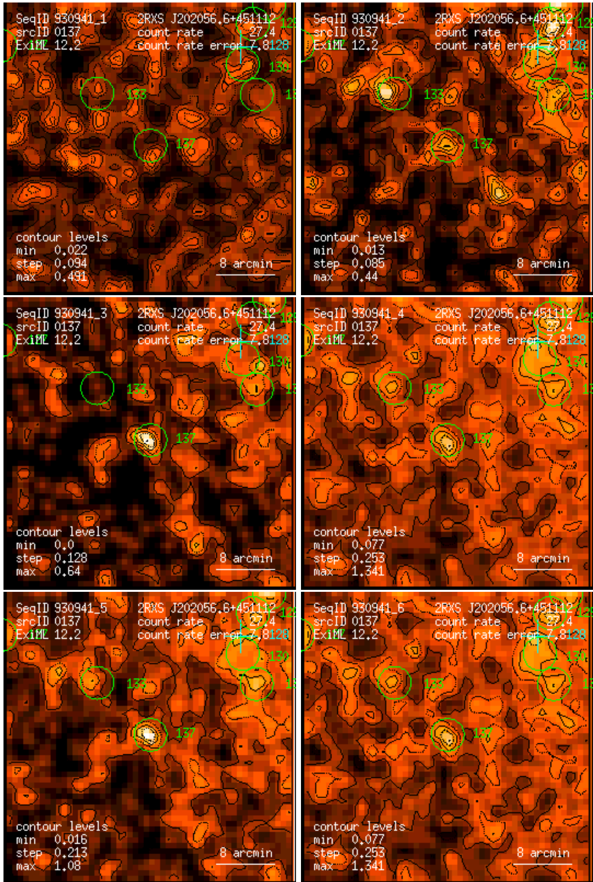
Figure 137: RASS 930941: detection 0137: band rate images, Gaussian filter: (1) PSPC channels 11 – 41, (2) 52 – 90, (3) 91 – 201, (4) 11 – 235, (5) 52 – 201, (6) 11 – 201. Broad band rates in counts/ks. Band rate contour levels in counts/ks/arcmin 2 .
