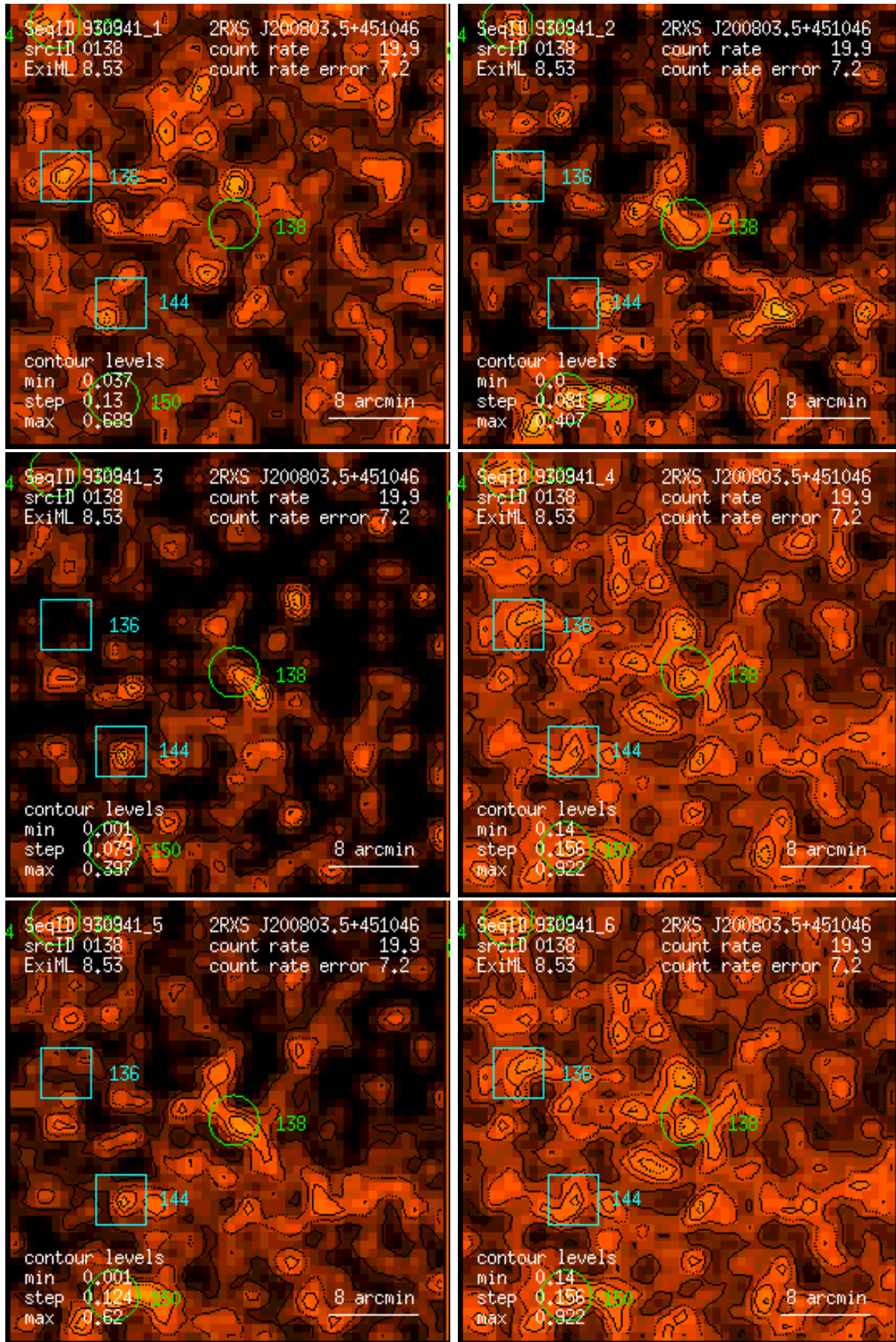
Figure 138: RASS 930941: detection 0138: band rate images, Gaussian filter: (1) PSPC channels 11 – 41, (2) 52 – 90, (3) 91 – 201, (4) 11 – 235, (5) 52 – 201, (6) 11 – 201. Broad band rates in counts/ks. Band rate contour levels in counts/ks/arcmin 2 .
