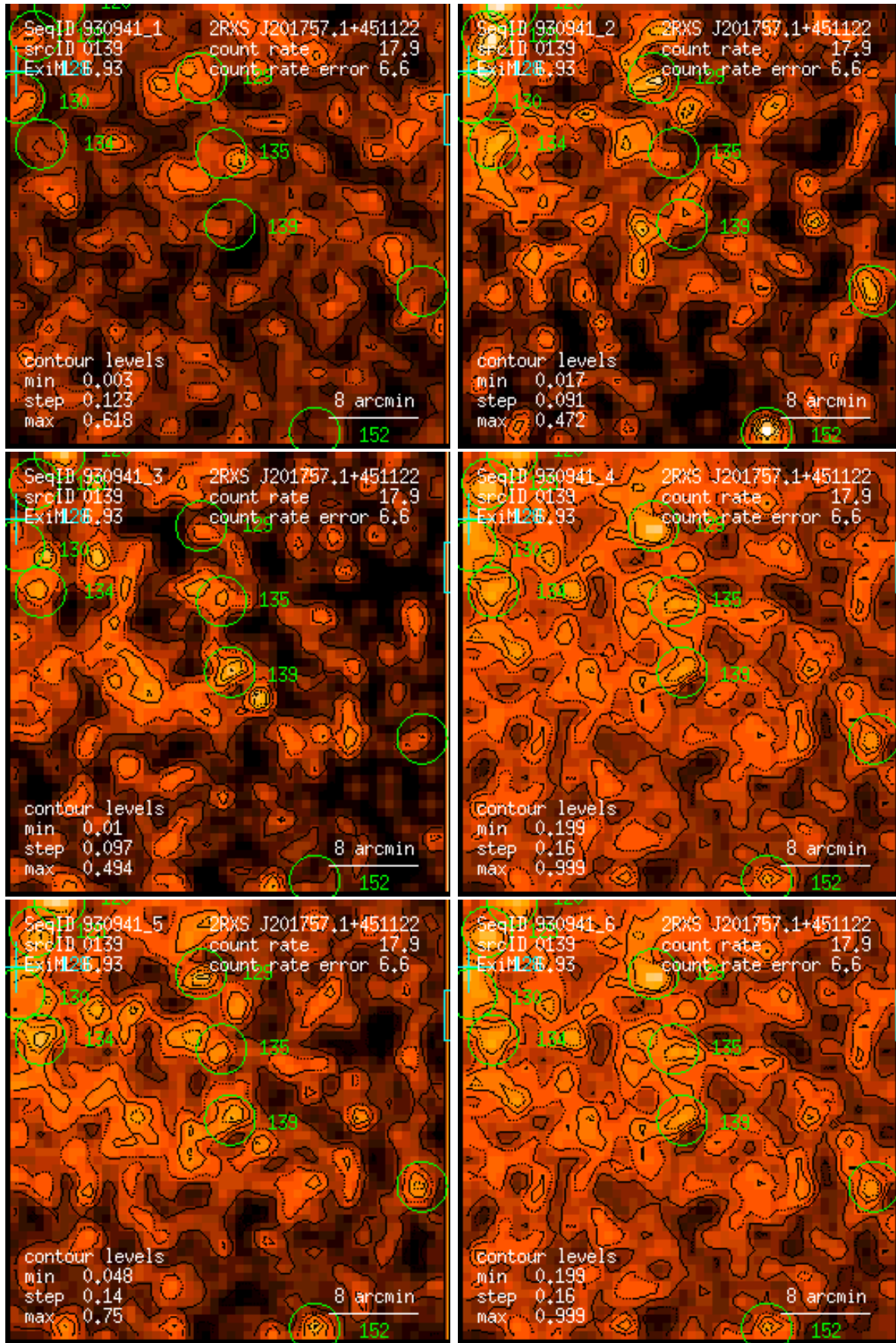
Figure 139: RASS 930941: detection 0139: band rate images, Gaussian filter: (1) PSPC channels 11 – 41, (2) 52 – 90, (3) 91 – 201, (4) 11 – 235, (5) 52 – 201, (6) 11 – 201. Broad band rates in counts/ks. Band rate contour levels in counts/ks/arcmin 2 .
