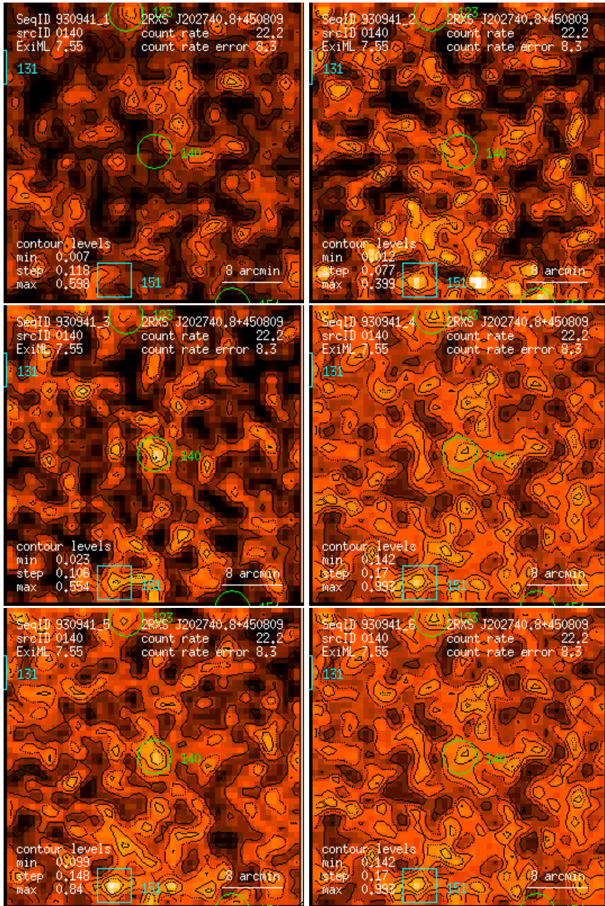
Figure 140: RASS 930941: detection 0140: band rate images, Gaussian filter: (1) PSPC channels 11 – 41, (2) 52 – 90, (3) 91 – 201, (4) 11 – 235, (5) 52 – 201, (6) 11 – 201. Broad band rates in counts/ks. Band rate contour levels in counts/ks/arcmin 2 .
