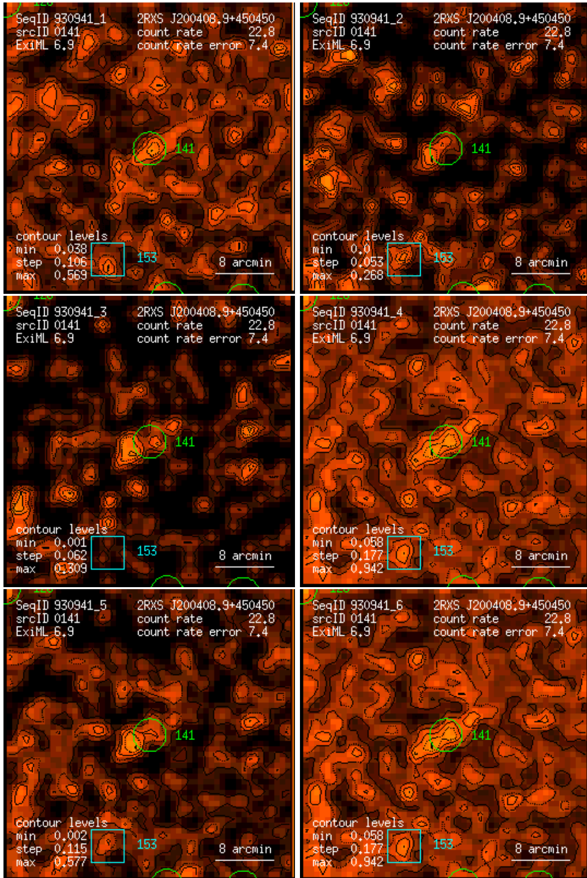
Figure 141: RASS 930941: detection 0141: band rate images, Gaussian filter: (1) PSPC channels 11 – 41, (2) 52 – 90, (3) 91 – 201, (4) 11 – 235, (5) 52 – 201, (6) 11 – 201. Broad band rates in counts/ks. Band rate contour levels in counts/ks/arcmin 2 .
