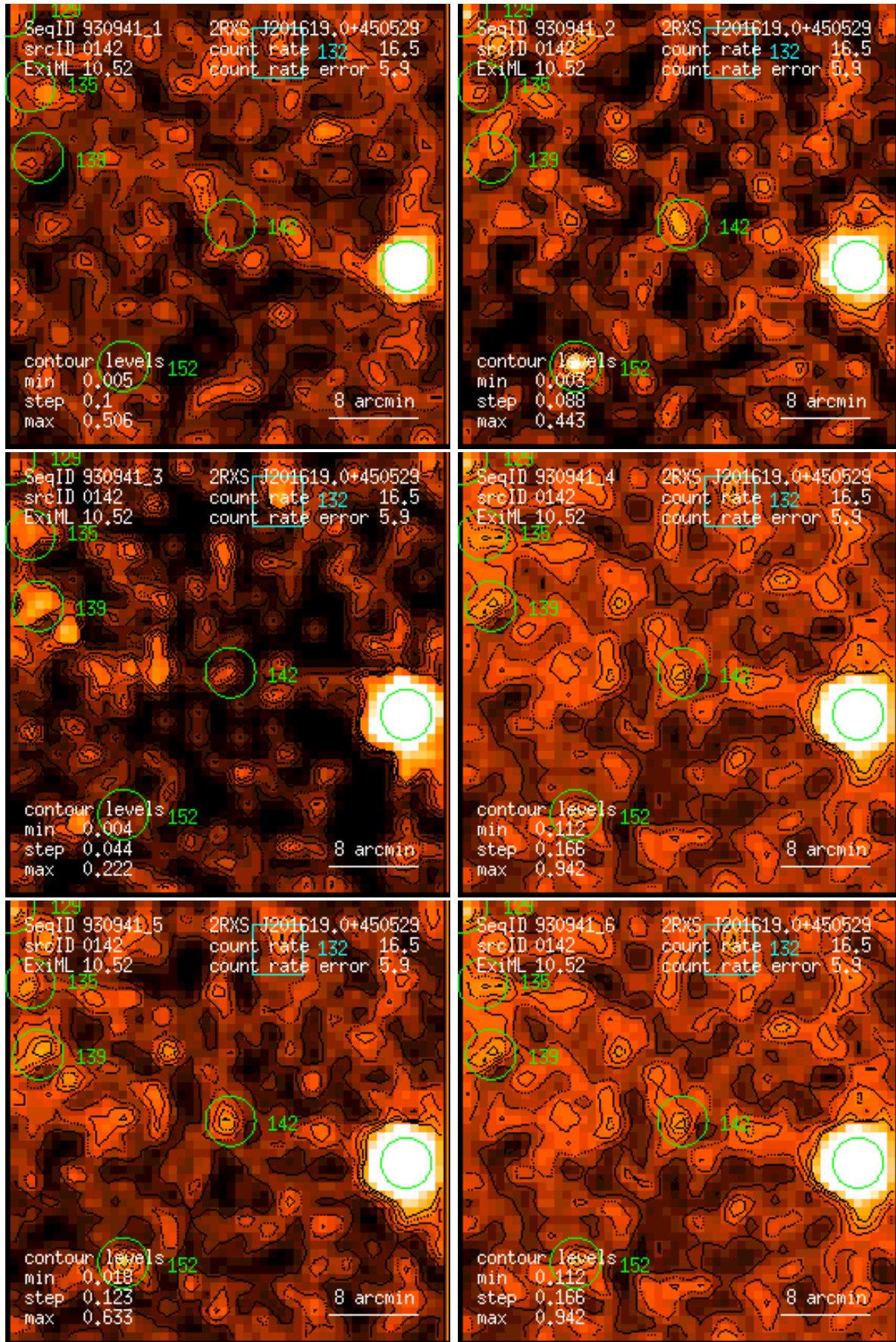
Figure 142: RASS 930941: detection 0142: band rate images, Gaussian filter: (1) PSPC channels 11 – 41, (2) 52 – 90, (3) 91 – 201, (4) 11 – 235, (5) 52 – 201, (6) 11 – 201. Broad band rates in counts/ks. Band rate contour levels in counts/ks/arcmin 2 .
