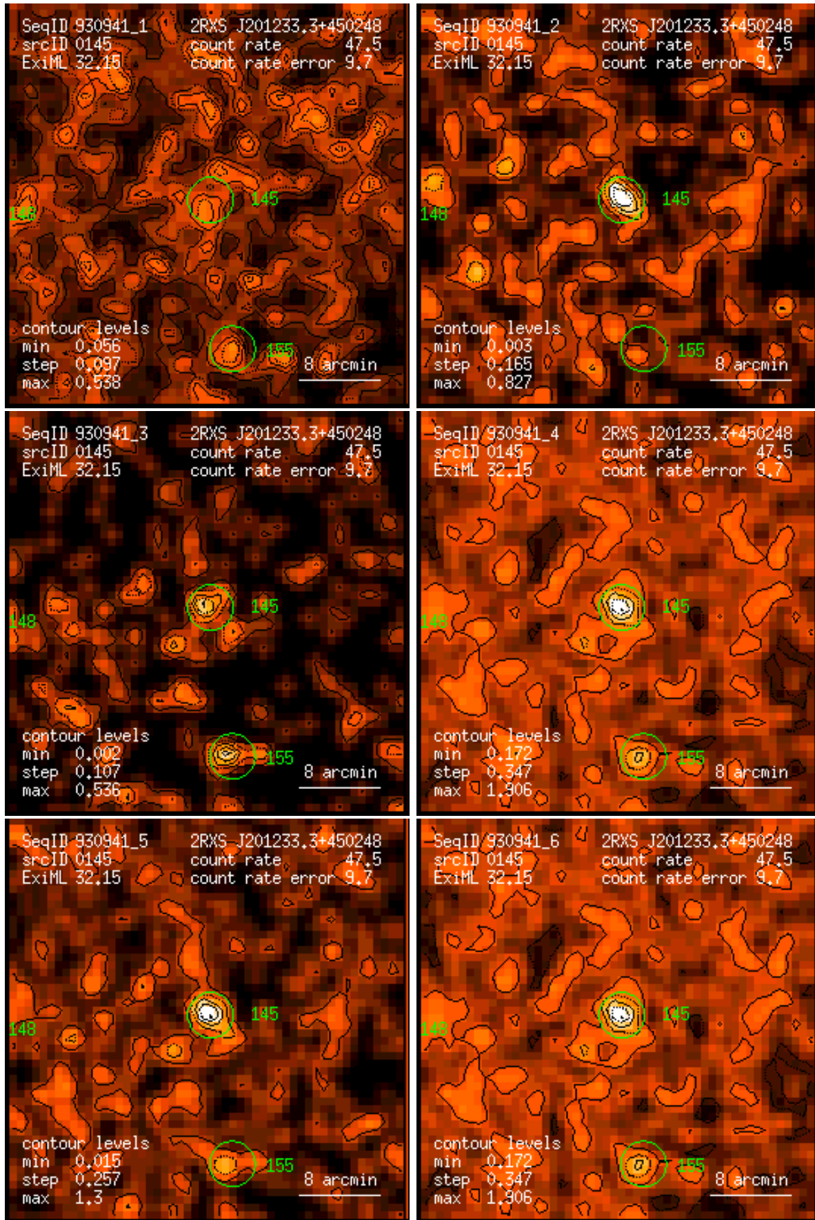
Figure 145: RASS 930941: detection 0145: band rate images, Gaussian filter: (1) PSPC channels 11 – 41, (2) 52 – 90, (3) 91 – 201, (4) 11 – 235, (5) 52 – 201, (6) 11 – 201. Broad band rates in counts/ks. Band rate contour levels in counts/ks/arcmin 2 .
