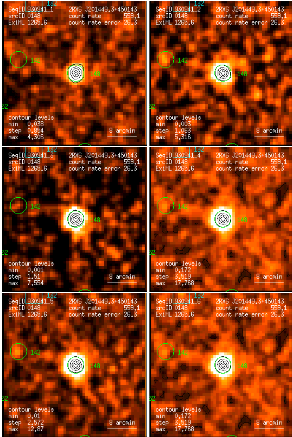
Figure 148: RASS 930941: detection 0148: band rate images, Gaussian filter: (1) PSPC channels 11 – 41, (2) 52 – 90, (3) 91 – 201, (4) 11 – 235, (5) 52 – 201, (6) 11 – 201. Broad band rates in counts/ks. Band rate contour levels in counts/ks/arcmin 2 .
