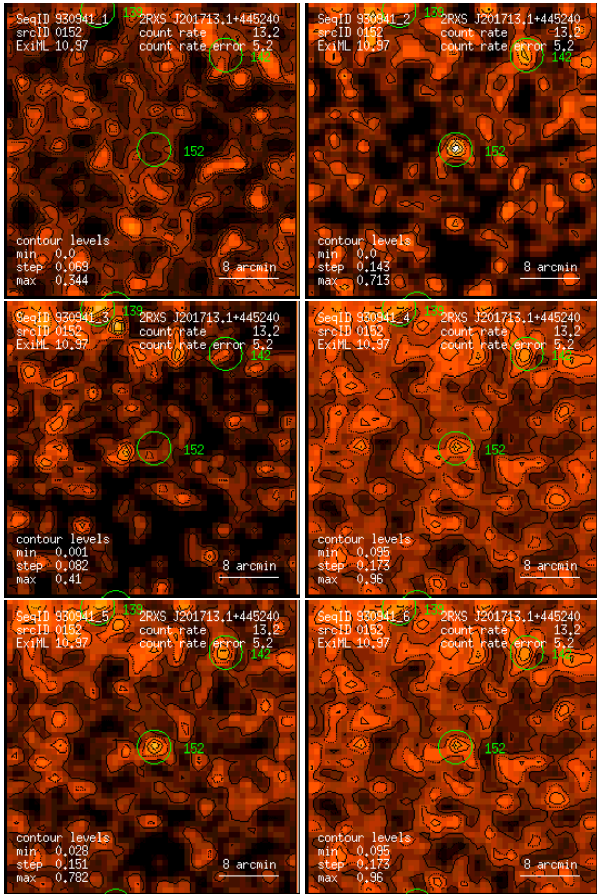
Figure 152: RASS 930941: detection 0152: band rate images, Gaussian filter: (1) PSPC channels 11 – 41, (2) 52 – 90, (3) 91 – 201, (4) 11 – 235, (5) 52 – 201, (6) 11 – 201. Broad band rates in counts/ks. Band rate contour levels in counts/ks/arcmin 2 .
