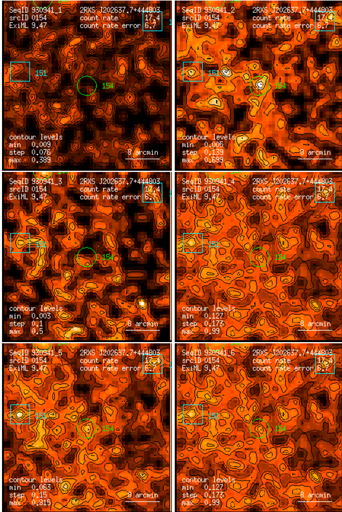
Figure 154: RASS 930941: detection 0154: band rate images, Gaussian filter: (1) PSPC channels 11 – 41, (2) 52 – 90, (3) 91 – 201, (4) 11 – 235, (5) 52 – 201, (6) 11 – 201. Broad band rates in counts/ks. Band rate contour levels in counts/ks/arcmin 2 .
