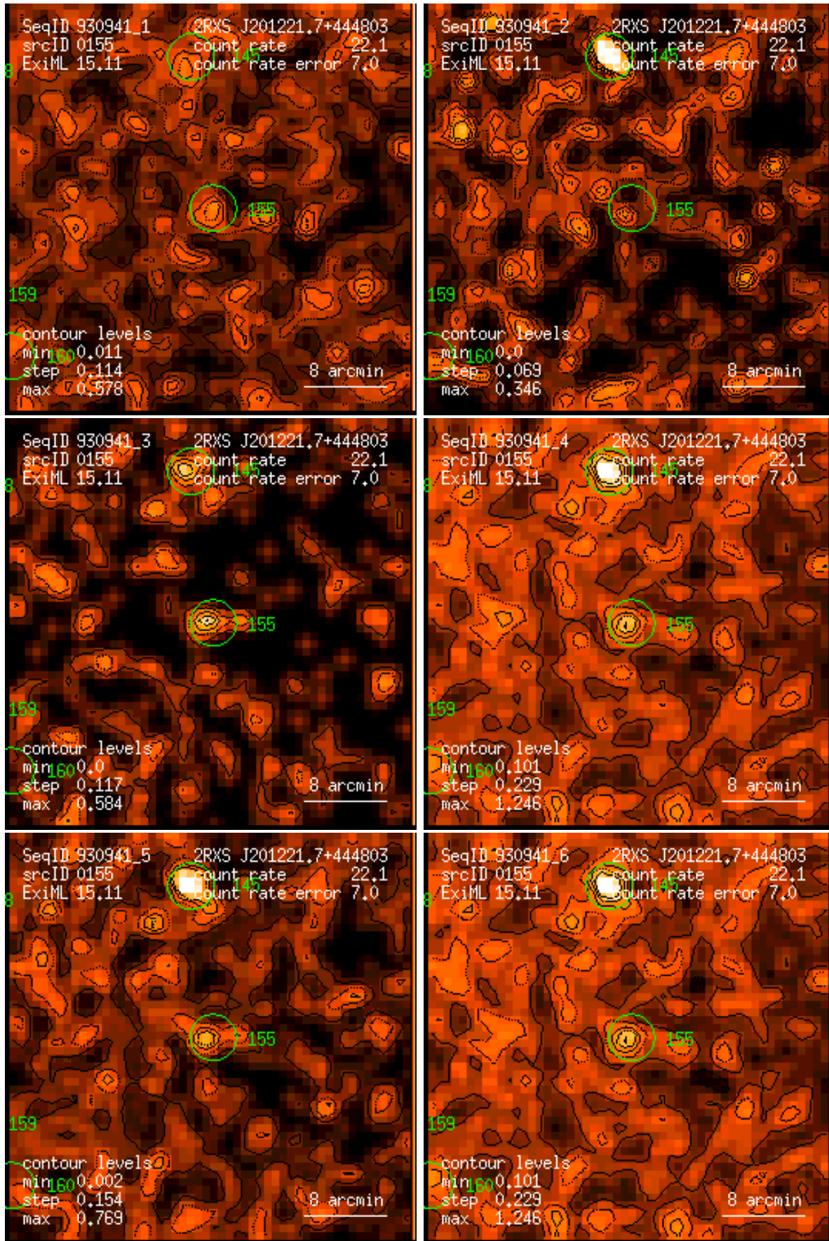
Figure 155: RASS 930941: detection 0155: band rate images, Gaussian filter: (1) PSPC channels 11 – 41, (2) 52 – 90, (3) 91 – 201, (4) 11 – 235, (5) 52 – 201, (6) 11 – 201. Broad band rates in counts/ks. Band rate contour levels in counts/ks/arcmin 2 .
