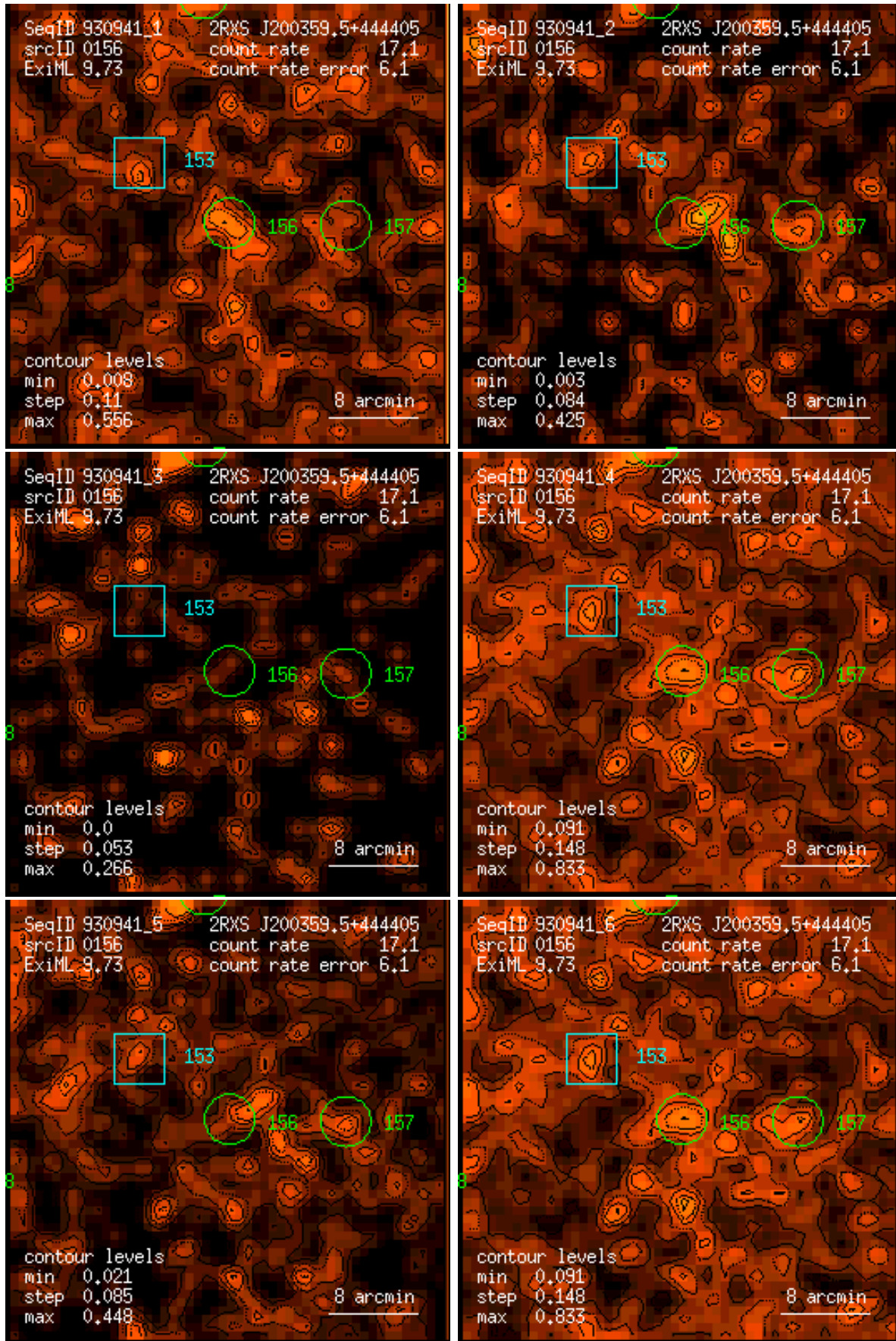
Figure 156: RASS 930941: detection 0156: band rate images, Gaussian filter: (1) PSPC channels 11 – 41, (2) 52 – 90, (3) 91 – 201, (4) 11 – 235, (5) 52 – 201, (6) 11 – 201. Broad band rates in counts/ks. Band rate contour levels in counts/ks/arcmin 2 .
