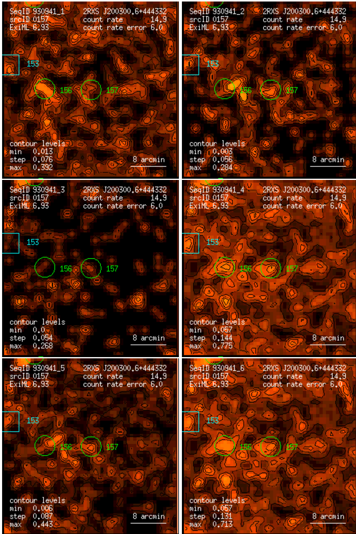
Figure 157: RASS 930941: detection 0157: band rate images, Gaussian filter: (1) PSPC channels 11 – 41, (2) 52 – 90, (3) 91 – 201, (4) 11 – 235, (5) 52 – 201, (6) 11 – 201. Broad band rates in counts/ks. Band rate contour levels in counts/ks/arcmin 2 .
