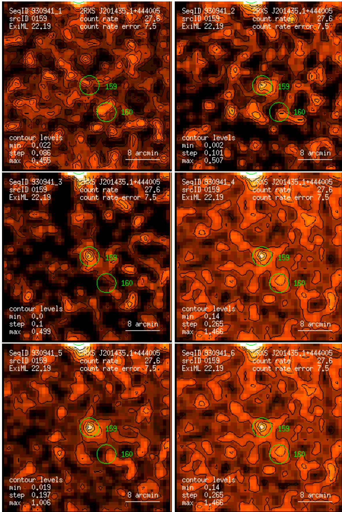
Figure 159: RASS 930941: detection 0159: band rate images, Gaussian filter: (1) PSPC channels 11 – 41, (2) 52 – 90, (3) 91 – 201, (4) 11 – 235, (5) 52 – 201, (6) 11 – 201. Broad band rates in counts/ks. Band rate contour levels in counts/ks/arcmin 2 .
