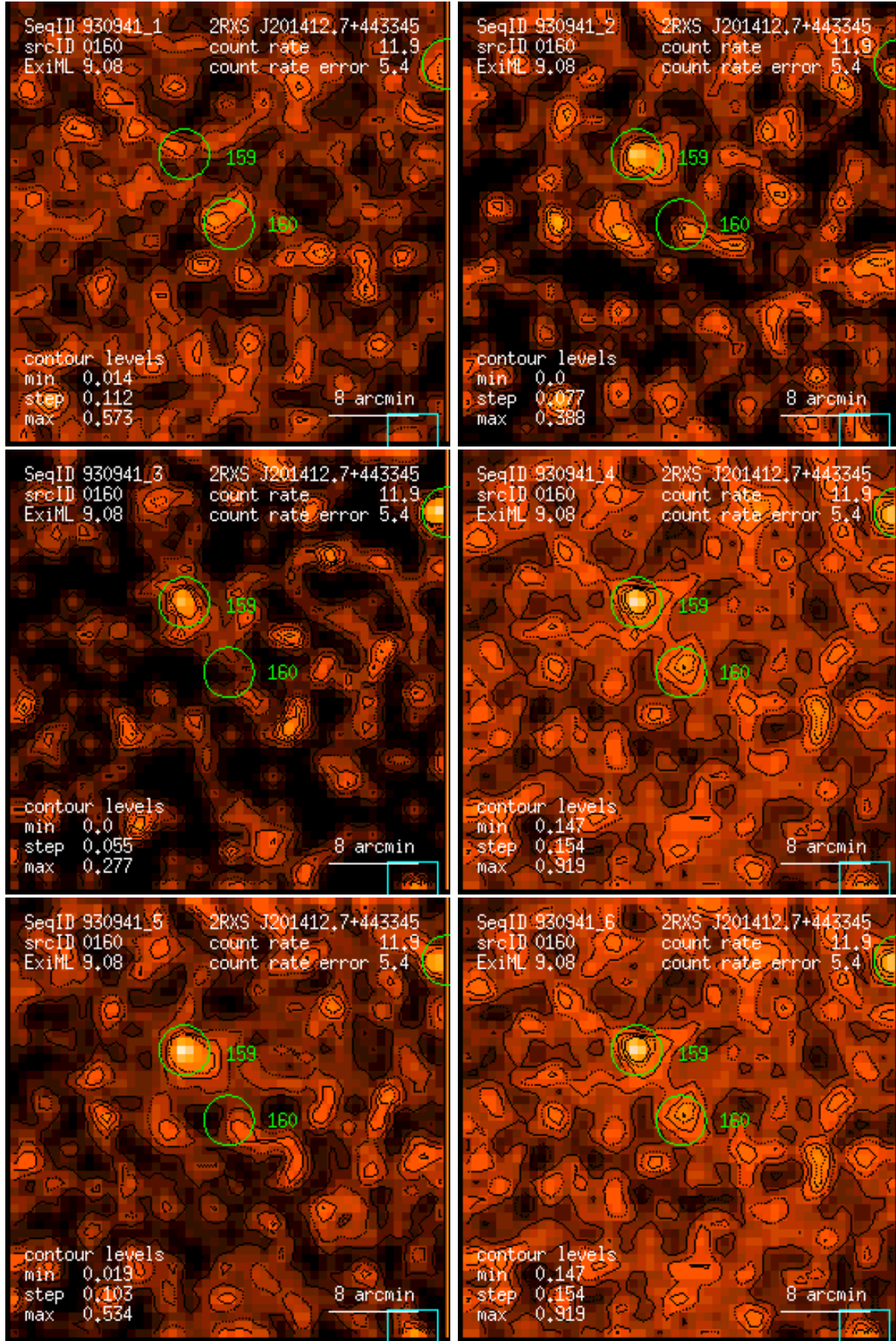
Figure 160: RASS 930941: detection 0160: band rate images, Gaussian filter: (1) PSPC channels 11 – 41, (2) 52 – 90, (3) 91 – 201, (4) 11 – 235, (5) 52 – 201, (6) 11 – 201. Broad band rates in counts/ks. Band rate contour levels in counts/ks/arcmin 2 .
