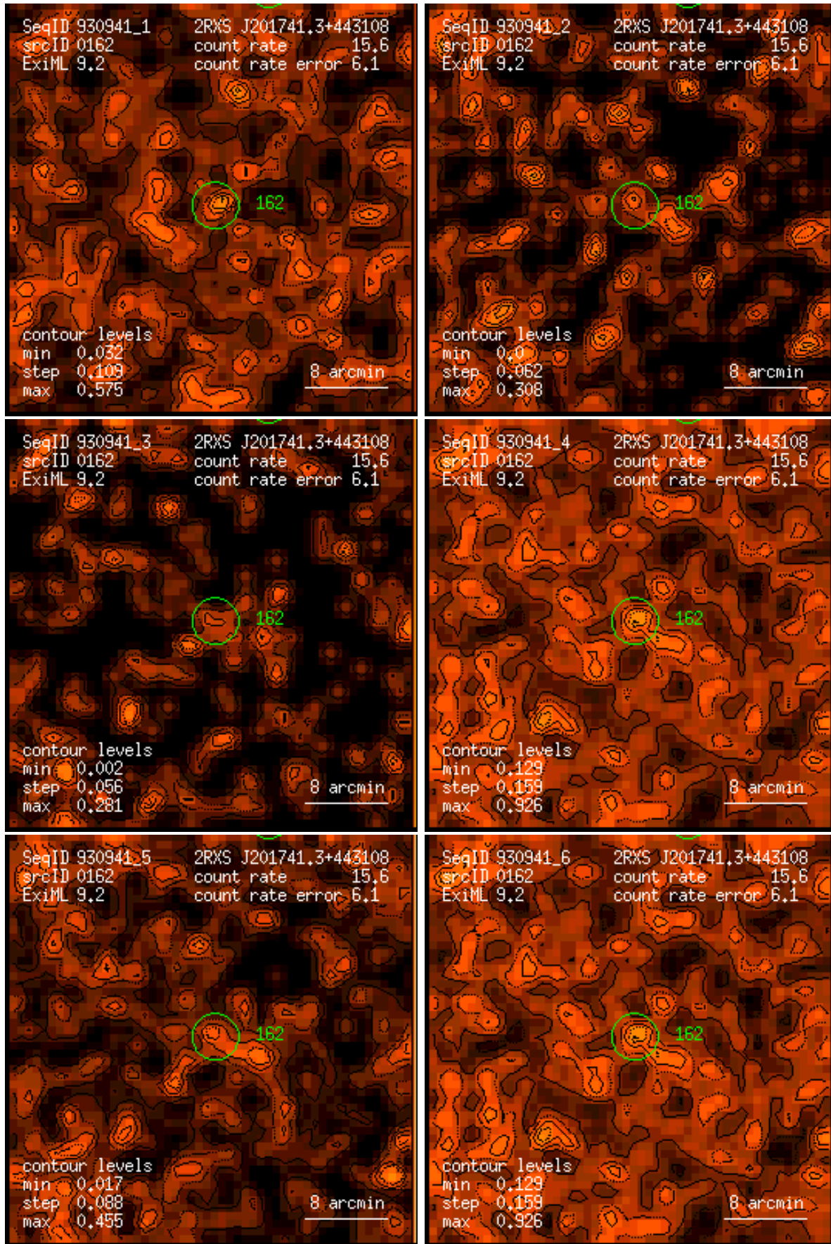
Figure 162: RASS 930941: detection 0162: band rate images, Gaussian filter: (1) PSPC channels 11 – 41, (2) 52 – 90, (3) 91 – 201, (4) 11 – 235, (5) 52 – 201, (6) 11 – 201. Broad band rates in counts/ks. Band rate contour levels in counts/ks/arcmin 2 .
