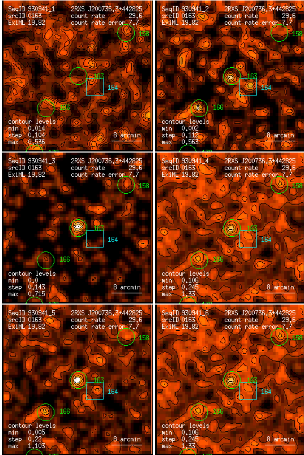
Figure 163: RASS 930941: detection 0163: band rate images, Gaussian filter: (1) PSPC channels 11 – 41, (2) 52 – 90, (3) 91 – 201, (4) 11 – 235, (5) 52 – 201, (6) 11 – 201. Broad band rates in counts/ks. Band rate contour levels in counts/ks/arcmin 2 .
