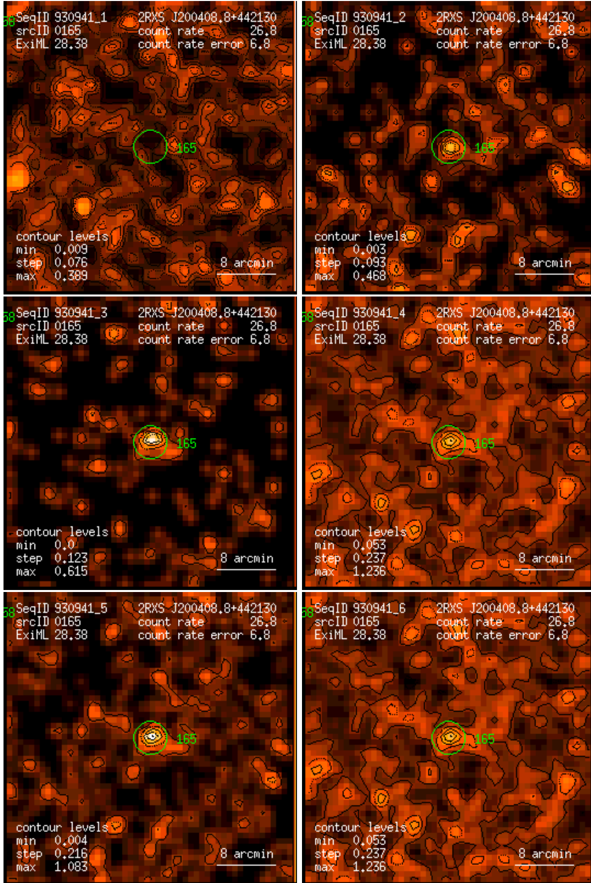
Figure 165: RASS 930941: detection 0165: band rate images, Gaussian filter: (1) PSPC channels 11 – 41, (2) 52 – 90, (3) 91 – 201, (4) 11 – 235, (5) 52 – 201, (6) 11 – 201. Broad band rates in counts/ks. Band rate contour levels in counts/ks/arcmin 2 .
