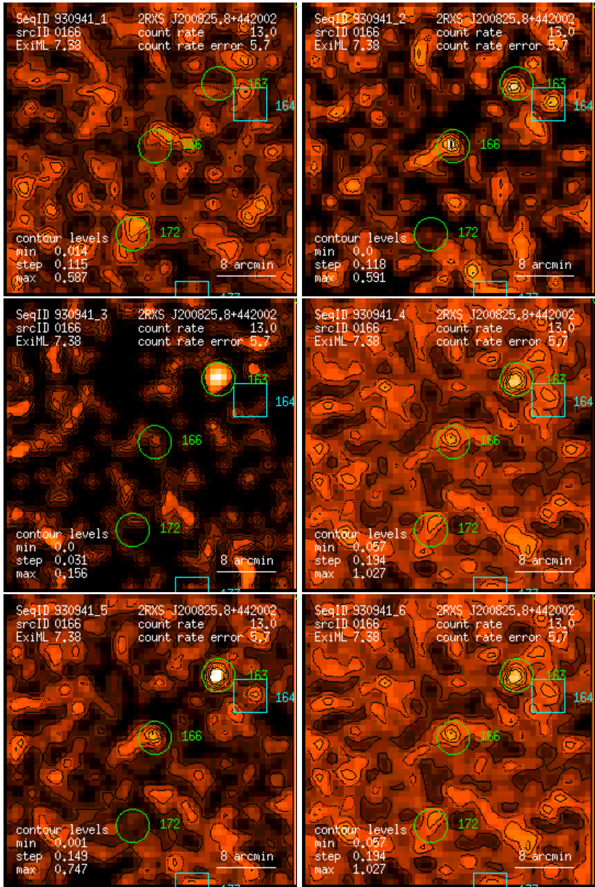
Figure 166: RASS 930941: detection 0166: band rate images, Gaussian filter: (1) PSPC channels 11 – 41, (2) 52 – 90, (3) 91 – 201, (4) 11 – 235, (5) 52 – 201, (6) 11 – 201. Broad band rates in counts/ks. Band rate contour levels in counts/ks/arcmin 2 .
