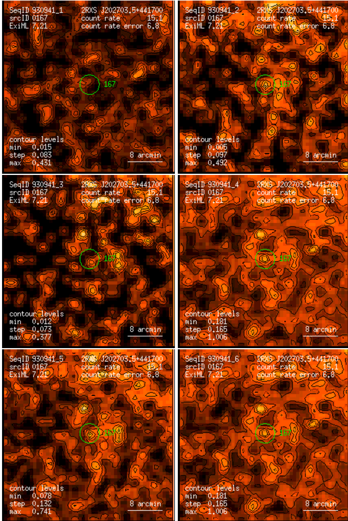
Figure 167: RASS 930941: detection 0167: band rate images, Gaussian filter: (1) PSPC channels 11 – 41, (2) 52 – 90, (3) 91 – 201, (4) 11 – 235, (5) 52 – 201, (6) 11 – 201. Broad band rates in counts/ks. Band rate contour levels in counts/ks/arcmin 2 .
