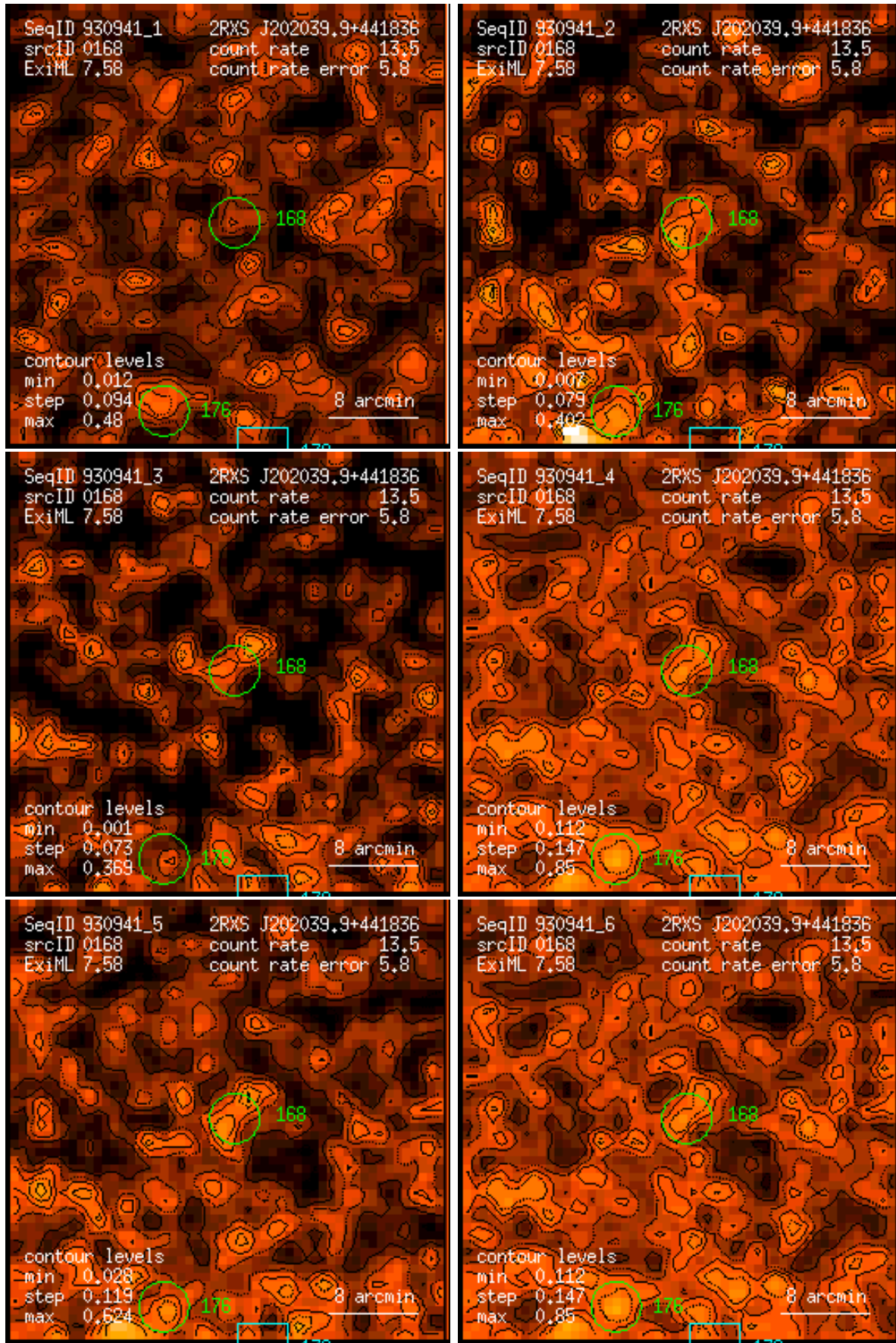
Figure 168: RASS 930941: detection 0168: band rate images, Gaussian filter: (1) PSPC channels 11 – 41, (2) 52 – 90, (3) 91 – 201, (4) 11 – 235, (5) 52 – 201, (6) 11 – 201. Broad band rates in counts/ks. Band rate contour levels in counts/ks/arcmin 2 .
