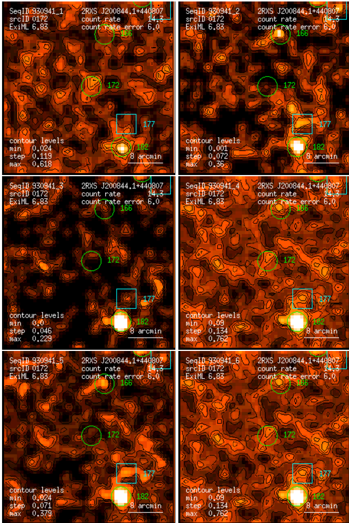
Figure 172: RASS 930941: detection 0172: band rate images, Gaussian filter: (1) PSPC channels 11 – 41, (2) 52 – 90, (3) 91 – 201, (4) 11 – 235, (5) 52 – 201, (6) 11 – 201. Broad band rates in counts/ks. Band rate contour levels in counts/ks/arcmin 2 .
