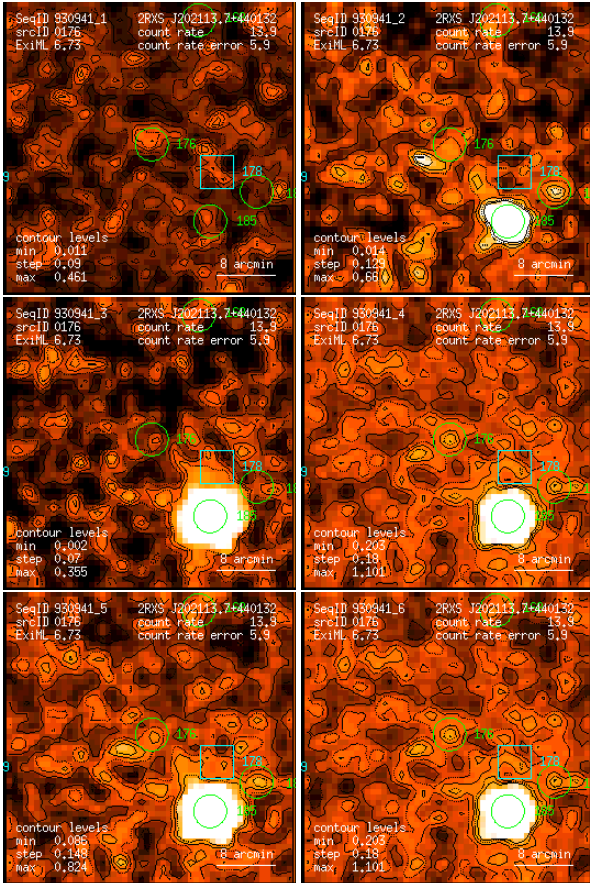
Figure 176: RASS 930941: detection 0176: band rate images, Gaussian filter: (1) PSPC channels 11 – 41, (2) 52 – 90, (3) 91 – 201, (4) 11 – 235, (5) 52 – 201, (6) 11 – 201. Broad band rates in counts/ks. Band rate contour levels in counts/ks/arcmin 2 .
