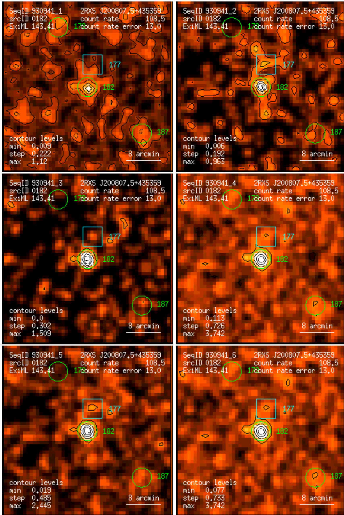
Figure 182: RASS 930941: detection 0182: band rate images, Gaussian filter: (1) PSPC channels 11 – 41, (2) 52 – 90, (3) 91 – 201, (4) 11 – 235, (5) 52 – 201, (6) 11 – 201. Broad band rates in counts/ks. Band rate contour levels in counts/ks/arcmin 2 .
