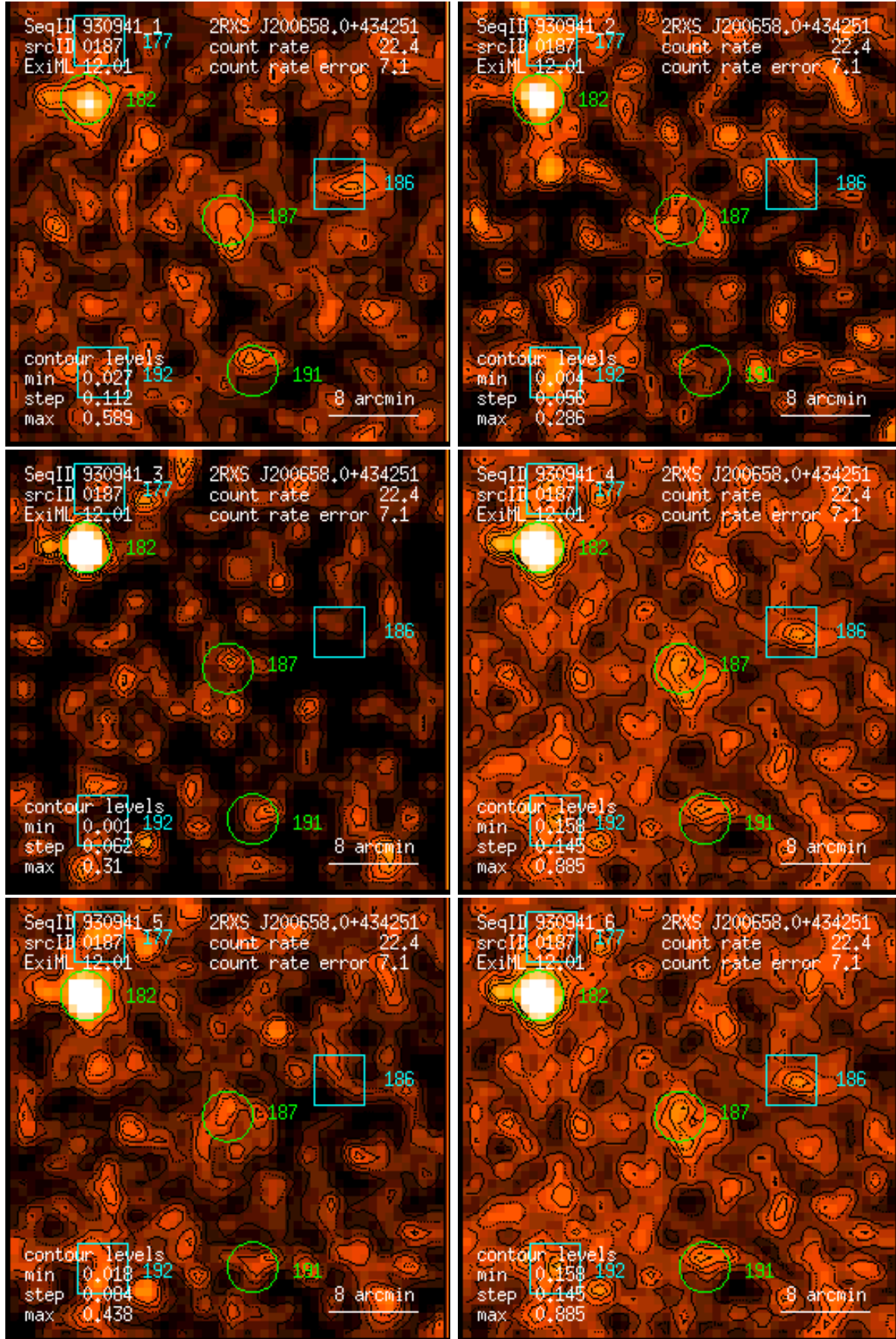
Figure 187: RASS 930941: detection 0187: band rate images, Gaussian filter: (1) PSPC channels 11 – 41, (2) 52 – 90, (3) 91 – 201, (4) 11 – 235, (5) 52 – 201, (6) 11 – 201. Broad band rates in counts/ks. Band rate contour levels in counts/ks/arcmin 2 .
