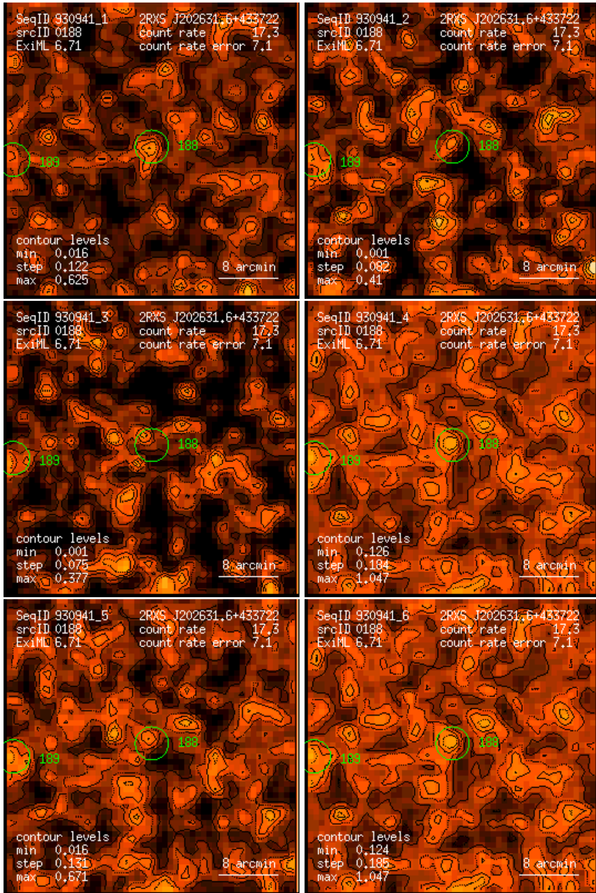
Figure 188: RASS 930941: detection 0188: band rate images, Gaussian filter: (1) PSPC channels 11 – 41, (2) 52 – 90, (3) 91 – 201, (4) 11 – 235, (5) 52 – 201, (6) 11 – 201. Broad band rates in counts/ks. Band rate contour levels in counts/ks/arcmin 2 .
