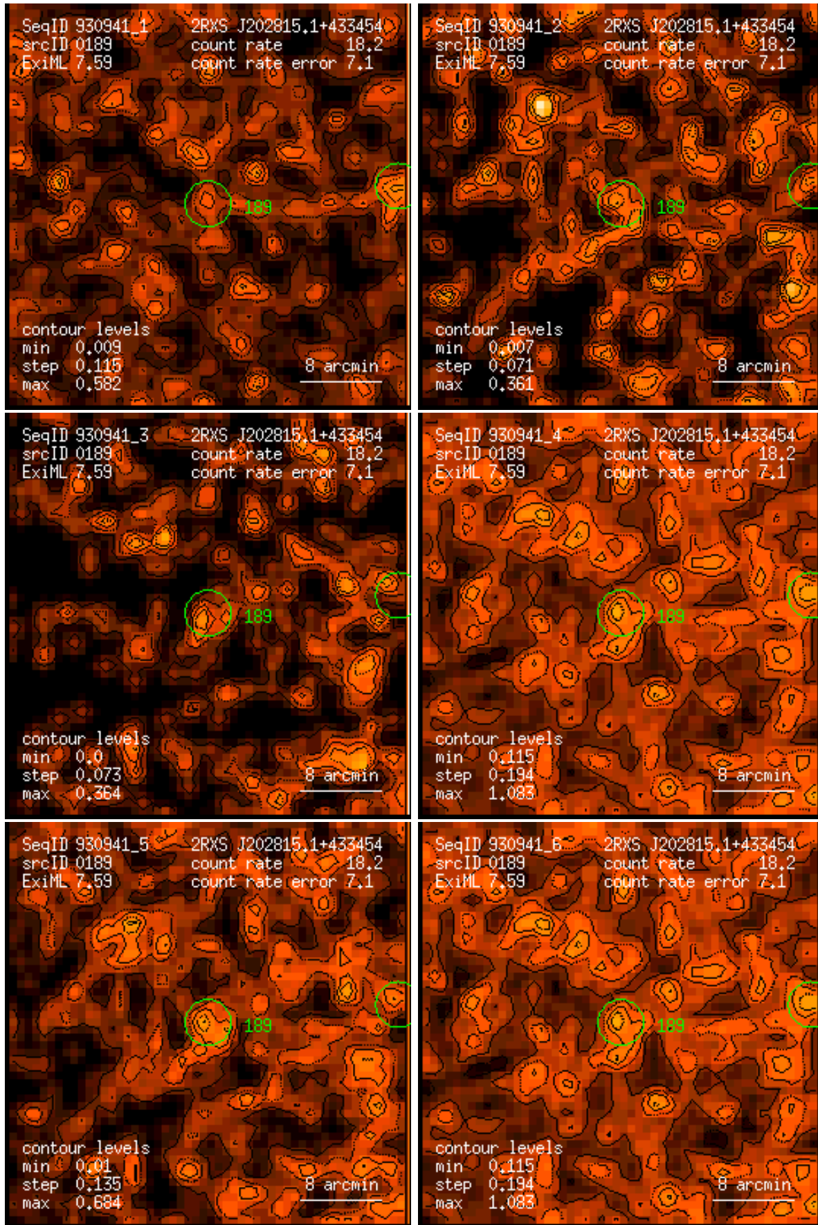
Figure 189: RASS 930941: detection 0189: band rate images, Gaussian filter: (1) PSPC channels 11 – 41, (2) 52 – 90, (3) 91 – 201, (4) 11 – 235, (5) 52 – 201, (6) 11 – 201. Broad band rates in counts/ks. Band rate contour levels in counts/ks/arcmin 2 .
