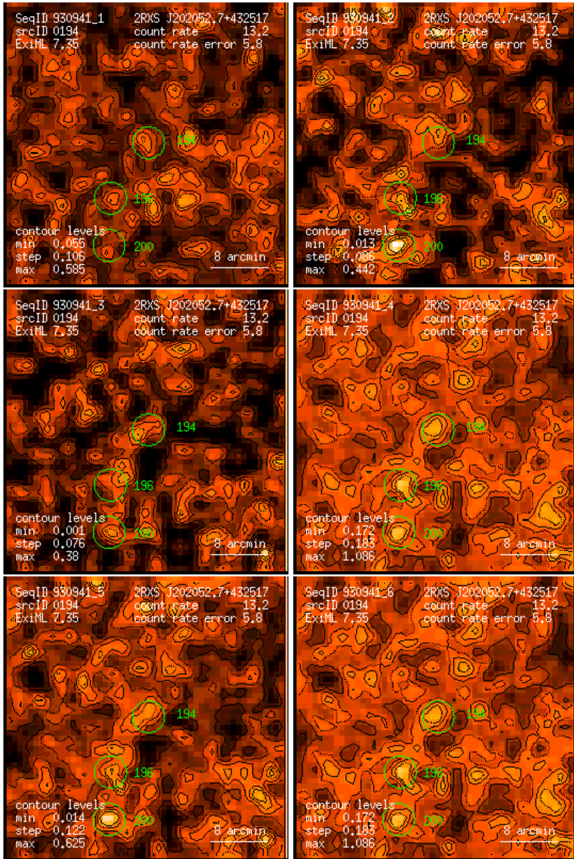
Figure 194: RASS 930941: detection 0194: band rate images, Gaussian filter: (1) PSPC channels 11 – 41, (2) 52 – 90, (3) 91 – 201, (4) 11 – 235, (5) 52 – 201, (6) 11 – 201. Broad band rates in counts/ks. Band rate contour levels in counts/ks/arcmin 2 .
