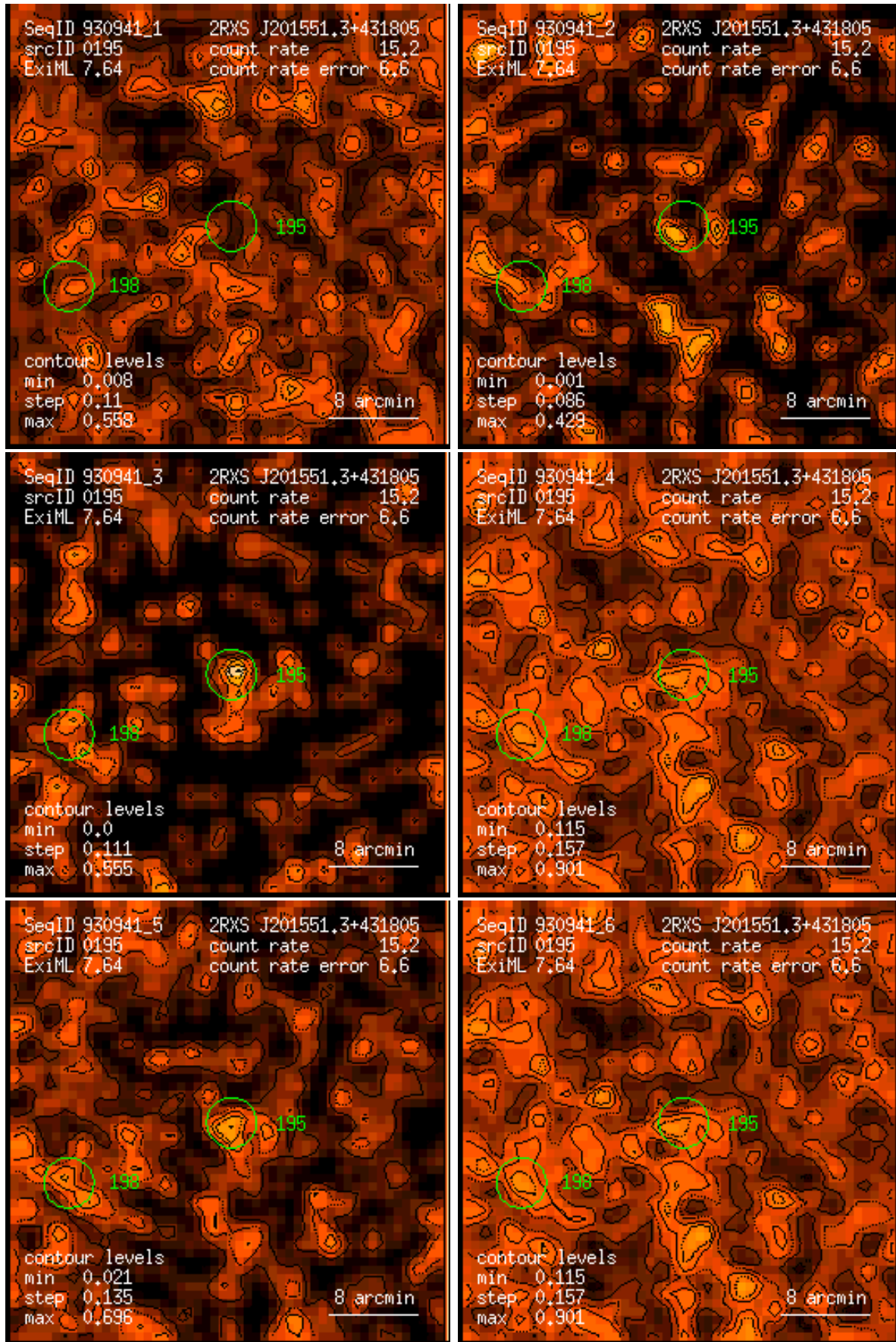
Figure 195: RASS 930941: detection 0195: band rate images, Gaussian filter: (1) PSPC channels 11 – 41, (2) 52 – 90, (3) 91 – 201, (4) 11 – 235, (5) 52 – 201, (6) 11 – 201. Broad band rates in counts/ks. Band rate contour levels in counts/ks/arcmin 2 .
