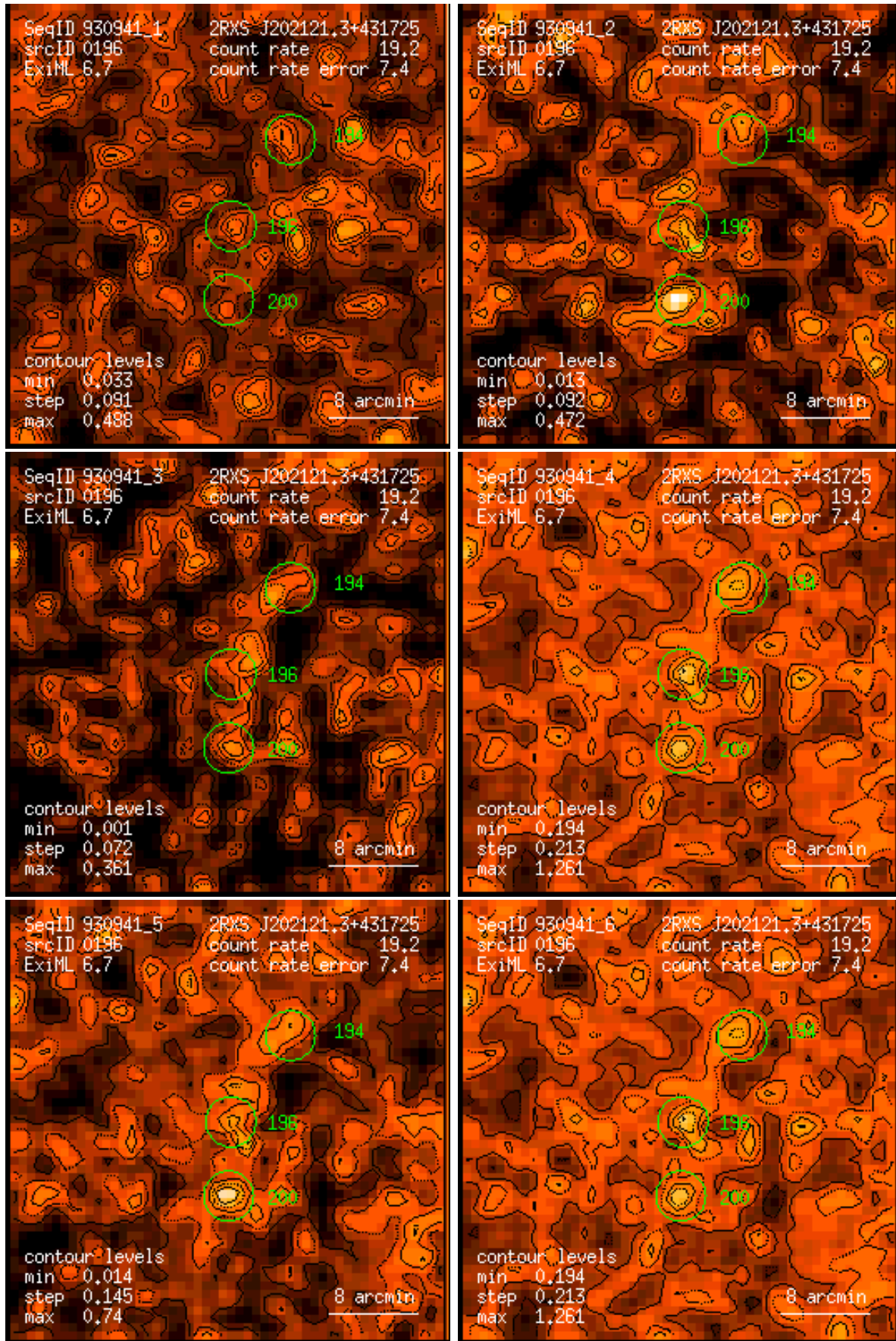
Figure 196: RASS 930941: detection 0196: band rate images, Gaussian filter: (1) PSPC channels 11 – 41, (2) 52 – 90, (3) 91 – 201, (4) 11 – 235, (5) 52 – 201, (6) 11 – 201. Broad band rates in counts/ks. Band rate contour levels in counts/ks/arcmin 2 .
